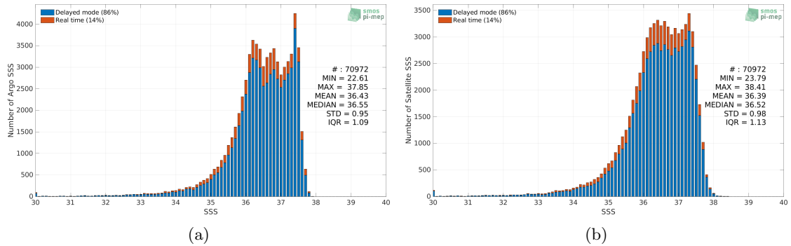
Figure 2: Histograms of SSS from Argo (a) and SMOS SSS L3 v8 - 9 Days (CATDS-CECOS-LOCEAN) (b) considering all match-up pairs per bins of 0.1 over the Amazon and Orinoco river plumes Pi-MEP region and for the full satellite product period.
