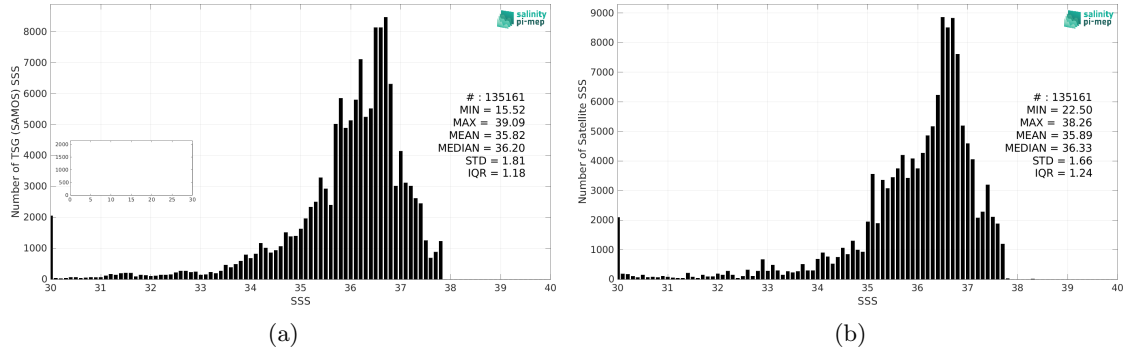
Figure 2: Histograms of SSS from TSG (SAMOS) (a) and SMOS SSS L3 v8 - 18 Days (CATDS-CEC-LOCEAN) (b) considering all match-up pairs per bins of 0.1 over the Amazon and Orinoco river plumes Pi-MEP region and for the full satellite product period.
