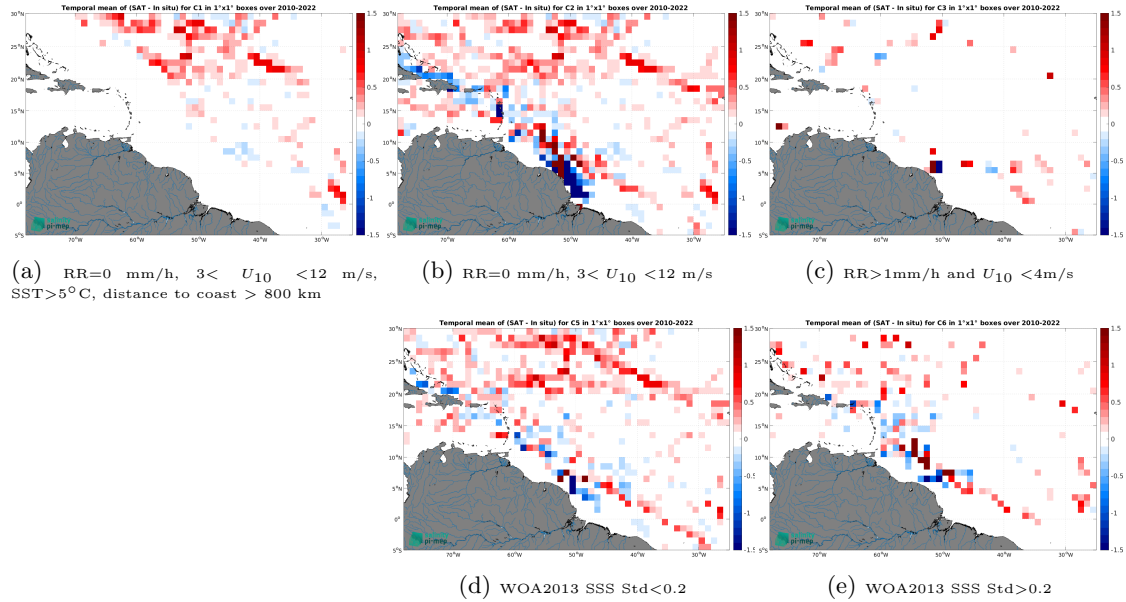
Figure 12: Temporal mean gridded over spatial boxes of size 1^{\circ}\times 1^{\circ} of \Delta\text{SSS} (SMOS SSS L3 v8 - 18 Days (CATDS-CEC-LOCEAN) - TSG (SAMOS)) for 5 different subdatasets corresponding to:RR=0 mm/h, 3 < U_{10} < 12 m/s, SST >5^{\circ}\text{C} , distance to coast > 800 km (a), RR=0 mm/h, 3 < U_{10} < 12 m/s (b), RR >1 mm/h and U_{10} < 4 m/s (c), WOA2013 SSS Std <0.2 (d), WOA2013 SSS Std >0.2 (e).
