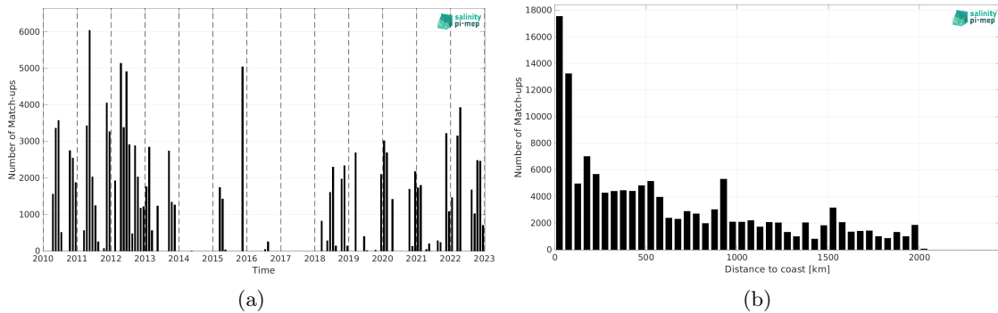
Figure 1: Number of match-ups between TSG (SAMOS) and SMOS SSS L3 v8 - 18 Days (CATDS-CEC-LOCEAN) SSS as a function of time (a) and as function of the distance to coast (b) over the Amazon and Orinoco river plumes Pi-MEP region and for the full satellite product period.
