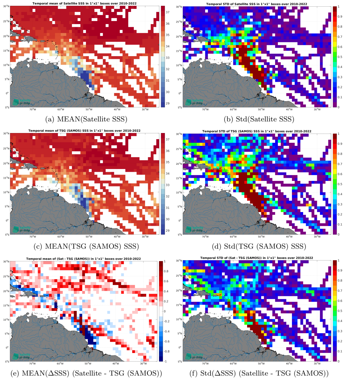
Figure 6: Temporal mean (left) and Std (right) of SSS from SMOS SSS L3 v8 - 18 Days (CATDS-CEC-LOCEAN) (top), TSG (SAMOS) (middle), and of \Delta SSS (Satellite - TSG (SAMOS)). Only match-up pairs are used to generate these maps.
