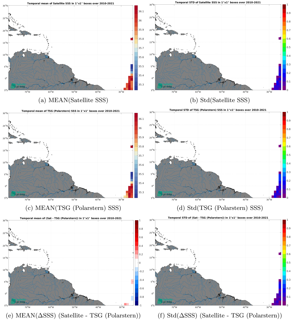
Figure 6: Temporal mean (left) and Std (right) of SSS from SMOS SSS L3 v8 - 18 Days (CATDS-CEC-LOCEAN) (top), TSG (Polarstern) (middle), and of \Delta SSS (Satellite - TSG (Polarstern)). Only match-up pairs are used to generate these maps.
