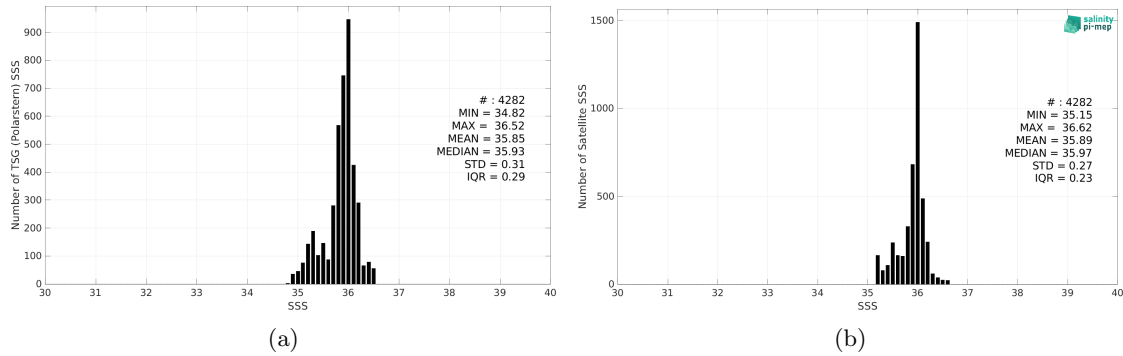
Figure 2: Histograms of SSS from TSG (Polarstern) (a) and SMOS SSS L3 v8 - 18 Days (CATDS-CEC-LOCEAN) (b) considering all match-up pairs per bins of 0.1 over the Amazon and Orinoco river plumes Pi-MEP region and for the full satellite product period.
