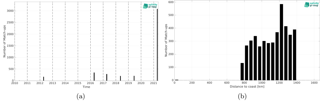
Figure 1: Number of match-ups between TSG (Polarstern) and SMOS SSS L3 v8 - 18 Days (CATDS-CEC-LOCEAN) SSS as a function of time (a) and as function of the distance to coast (b) over the Amazon and Orinoco river plumes Pi-MEP region and for the full satellite product period.
