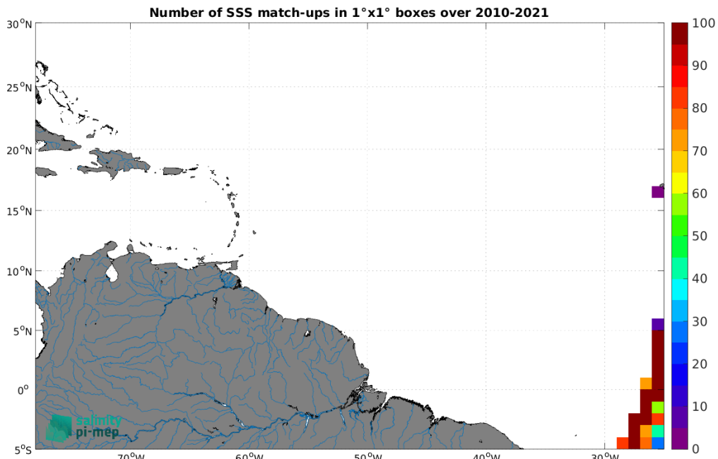
Figure 4: Number of SSS match-ups between TSG (Polarstern) SSS and the SMOS SSS L3 v8 - 18 Days (CATDS-CEC-LOCEAN) SSS product for the Amazon and Orinoco river plumes Pi-MEP region over 1^\circ \times 1^\circ boxes and for the full satellite product period.
