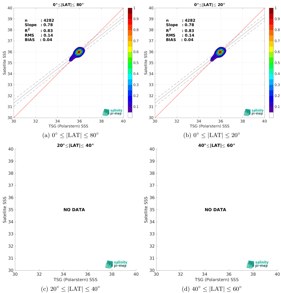
Figure 9: Contour maps of the concentration of SMOS SSS L3 v8 - 18 Days (CATDS-CEC-LOCEAN) SSS (y-axis) versus TSG (Polarstern) SSS (x-axis) at match-up pairs for different latitude bands. For each plot, the red line shows x=y . The black thin and dashed lines indicate a linear fit through the data cloud and the \pm 95\% confidence levels, respectively. The number match-up pairs n , the slope and R^2 coefficient of the linear fit, the root mean square (RMS) and the mean bias between satellite and in situ data are indicated for each latitude band in each plots.
