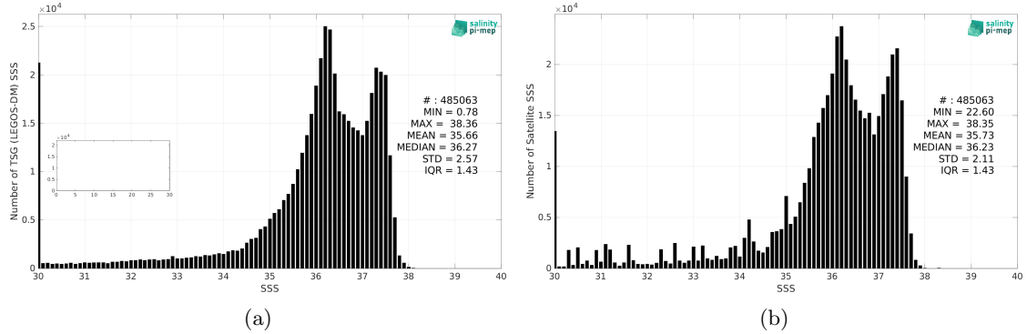
Figure 2: Histograms of SSS from TSG (LEGOS-DM) (a) and SMOS SSS L3 v8 - 18 Days (CATDS-CEC-LOCEAN) (b) considering all match-up pairs per bins of 0.1 over the Amazon and Orinoco river plumes Pi-MEP region and for the full satellite product period.
