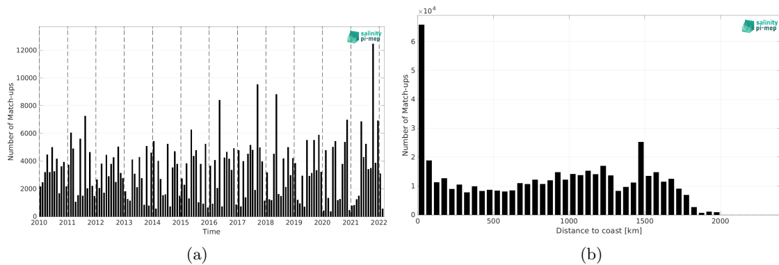
Figure 1: Number of match-ups between TSG (LEGOS-DM) and SMOS SSS L3 v8 - 18 Days (CATDS-CEC-LOCEAN) SSS as a function of time (a) and as function of the distance to coast (b) over the Amazon and Orinoco river plumes Pi-MEP region and for the full satellite product period.
