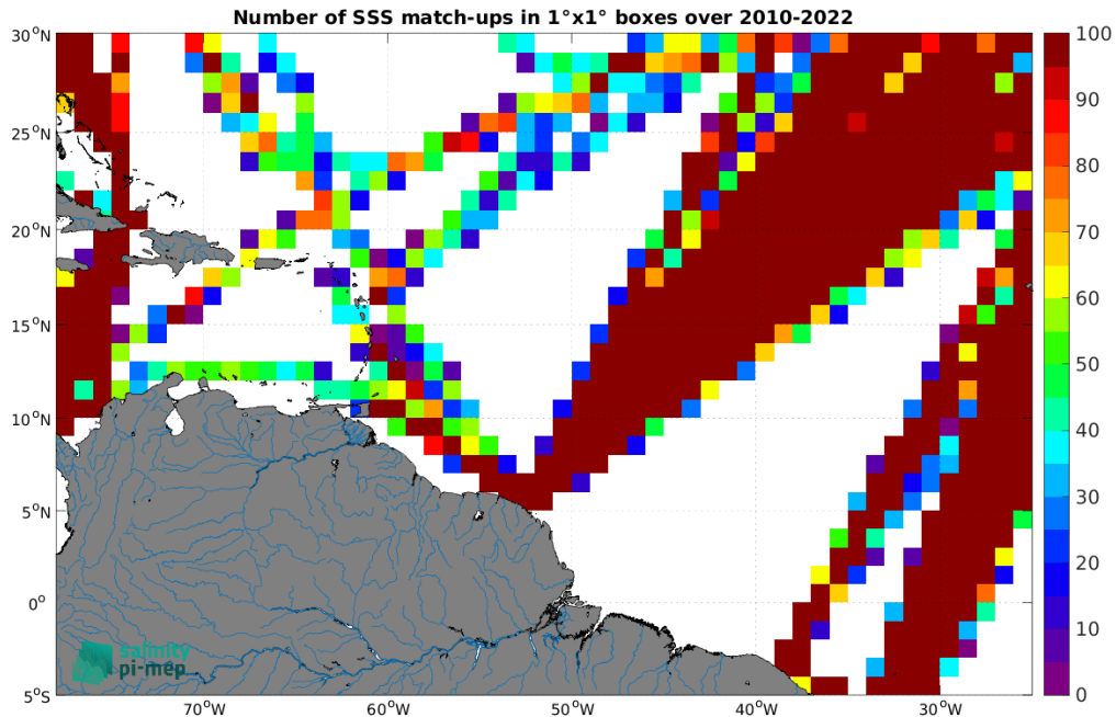
Figure 4: Number of SSS match-ups between TSG (LEGOS-DM) SSS and the SMOS SSS L3 v8 - 18 Days (CATDS-CEC-LOCEAN) SSS product for the Amazon and Orinoco river plumes Pi-MEP region over 1^\circ \times 1^\circ boxes and for the full satellite product period.
