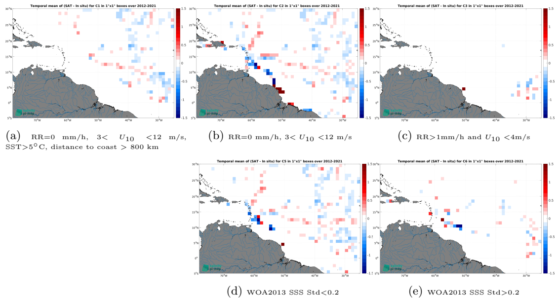
Figure 12: Temporal mean gridded over spatial boxes of size 1^{\circ}\times 1^{\circ} of \Delta SSS (SMOS SSS L3 v8 - 18 Days (CATDS-CEC-LOCEAN) - TSG (GOSUD-Sailing-ship)) for 5 different subdatasets corresponding to:RR=0 mm/h, 3 < U_{10} < 12 m/s, SST >5^{\circ}\text{C} , distance to coast > 800 km (a), RR=0 mm/h, 3 < U_{10} < 12 m/s (b), RR >1 mm/h and U_{10} < 4 m/s (c), WOA2013 SSS Std <0.2 (d), WOA2013 SSS Std >0.2 (e).
