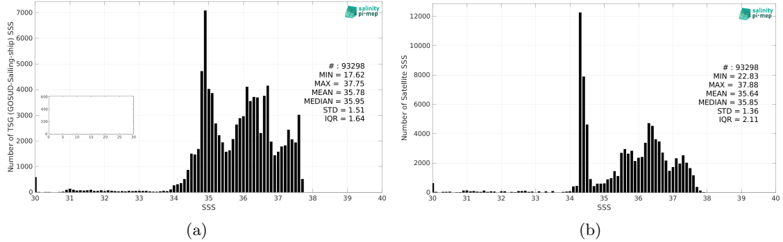
Figure 2: Histograms of SSS from TSG (GOSUD-Sailing-ship) (a) and SMOS SSS L3 v8 - 18 Days (CATDS-CEC-LOCEAN) (b) considering all match-up pairs per bins of 0.1 over the Amazon and Orinoco river plumes Pi-MEP region and for the full satellite product period.
