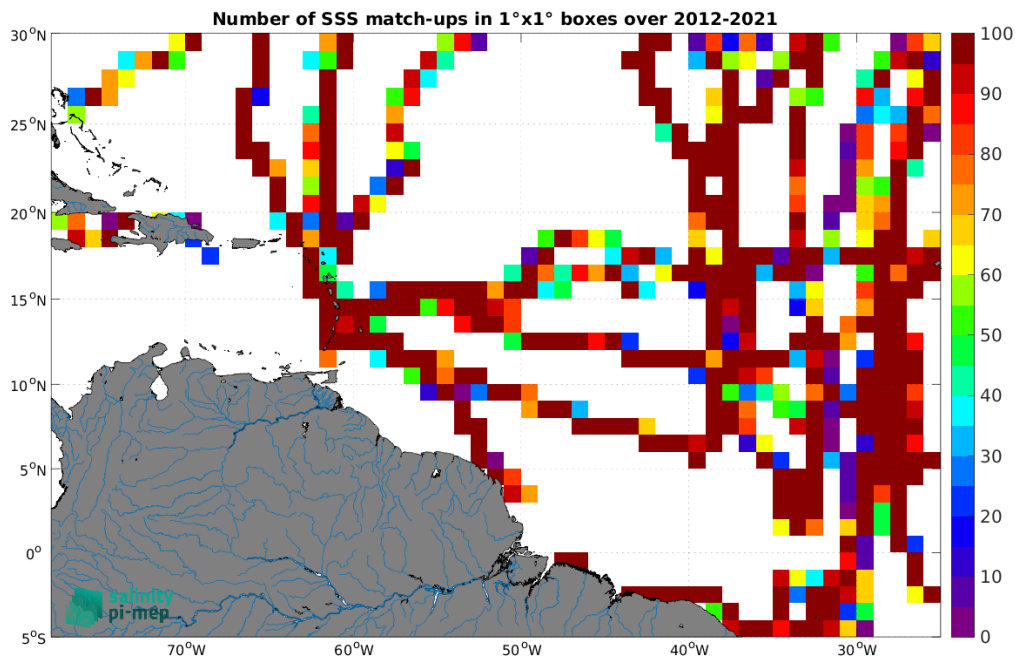
Figure 4: Number of SSS match-ups between TSG (GOSUD-Sailing-ship) SSS and the SMOS SSS L3 v8 - 18 Days (CATDS-CEC-LOCEAN) SSS product for the Amazon and Orinoco river plumes Pi-MEP region over 1^\circ \times 1^\circ boxes and for the full satellite product period.
