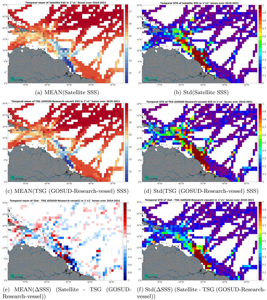
Figure 6: Temporal mean (left) and Std (right) of SSS from SMOS SSS L3 v8 - 18 Days (CATDS-CEC-LOCEAN) (top), TSG (GOSUD-Research-vessel) (middle), and of \Delta SSS (Satellite - TSG (GOSUD-Research-vessel)). Only match-up pairs are used to generate these maps.
