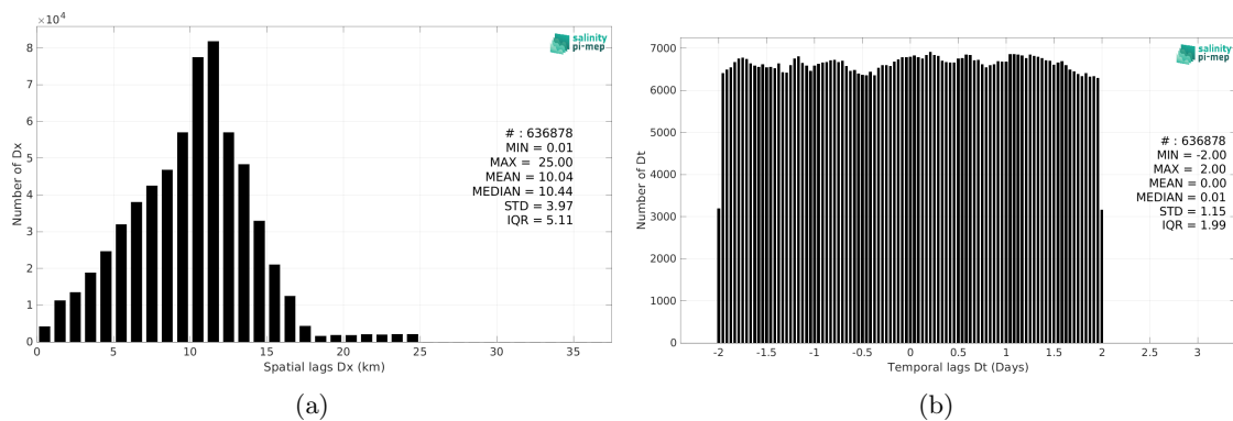
Figure 5: Histograms of the spatial (a) and temporal (b) lags between the location/time of the TSG (GOSUD-Research-vessel) measurement and the date of the corresponding SMOS SSS L3 v8 - 18 Days (CATDS-CEC-LOCEAN) SSS pixel.
