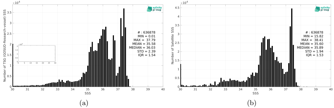
Figure 2: Histograms of SSS from TSG (GOSUD-Research-vessel) (a) and SMOS SSS L3 v8 - 18 Days (CATDS-CEC-LOCEAN) (b) considering all match-up pairs per bins of 0.1 over the Amazon and Orinoco river plumes Pi-MEP region and for the full satellite product period.
