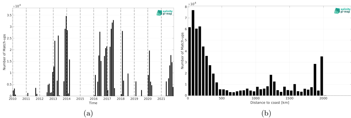
Figure 1: Number of match-ups between TSG (GOSUD-Research-vessel) and SMOS SSS L3 v8 - 18 Days (CATDS-CEC-LOCEAN) SSS as a function of time (a) and as function of the distance to coast (b) over the Amazon and Orinoco river plumes Pi-MEP region and for the full satellite product period.
