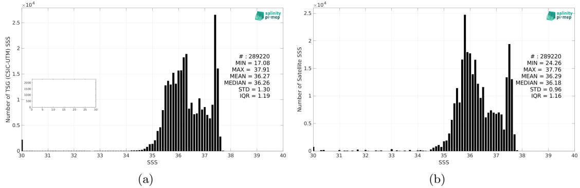
Figure 2: Histograms of SSS from TSG (CSIC-UTM) (a) and SMOS SSS L3 v8 - 18 Days (CATDS-CEC-LOCEAN) (b) considering all match-up pairs per bins of 0.1 over the Amazon and Orinoco river plumes Pi-MEP region and for the full satellite product period.
