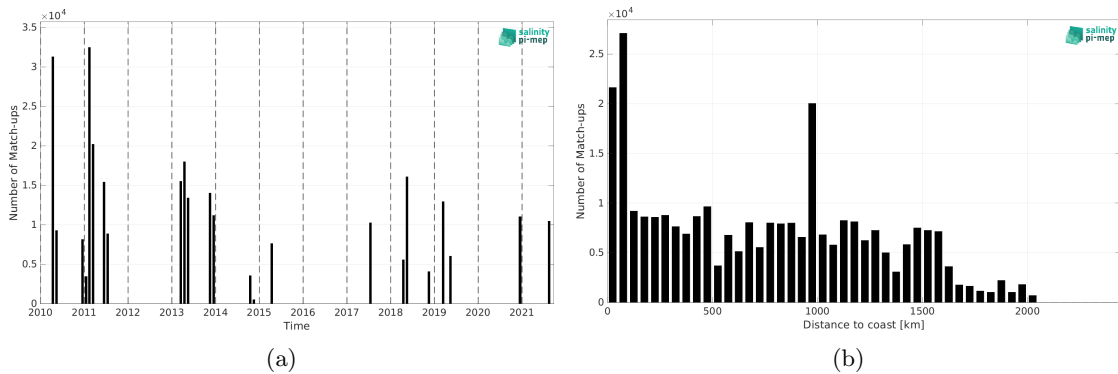
Figure 1: Number of match-ups between TSG (CSIC-UTM) and SMOS SSS L3 v8 - 18 Days (CATDS-CEC-LOCEAN) SSS as a function of time (a) and as function of the distance to coast (b) over the Amazon and Orinoco river plumes Pi-MEP region and for the full satellite product period.
