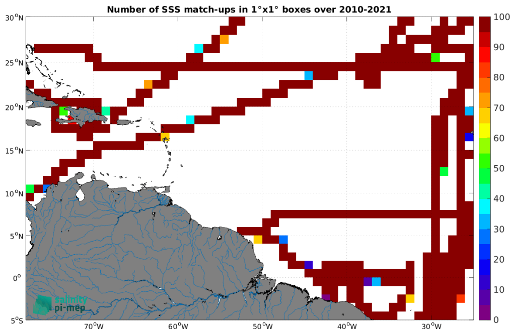
Figure 4: Number of SSS match-ups between TSG (CSIC-UTM) SSS and the SMOS SSS L3 v8 - 18 Days (CATDS-CEC-LOCEAN) SSS product for the Amazon and Orinoco river plumes Pi-MEP region over 1^\circ \times 1^\circ boxes and for the full satellite product period.
