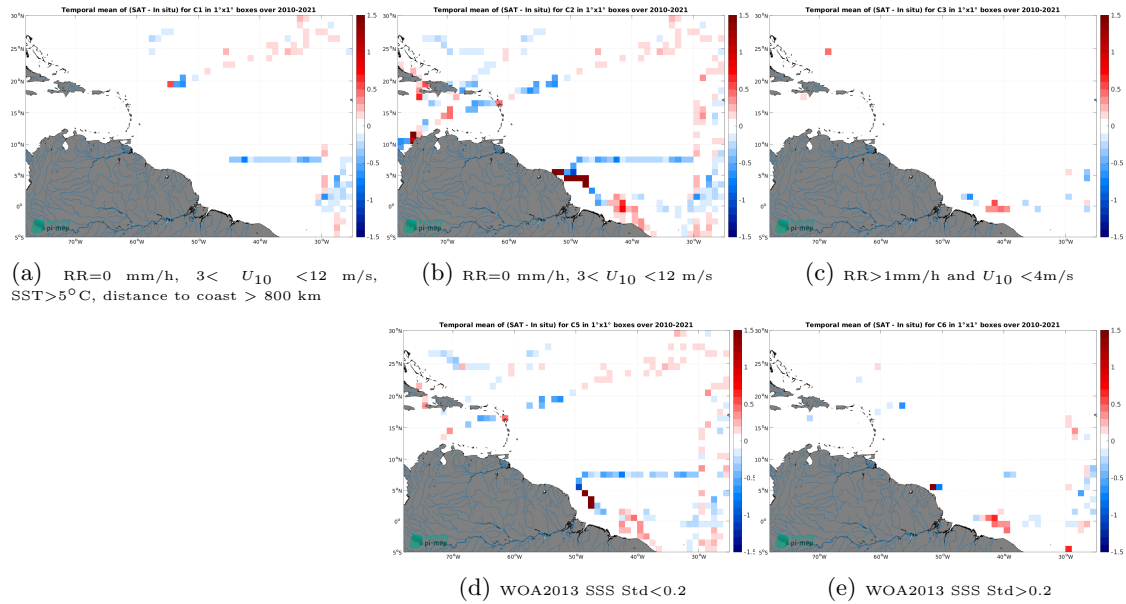
Figure 12: Temporal mean gridded over spatial boxes of size 1^\circ \times 1^\circ of \Delta SSS (SMOS SSS L3 v8 - 18 Days (CATDS-CEC-LOCEAN) - TSG (CSIC-UTM)) for 5 different subdatasets corresponding to:RR=0 mm/h, 3 < U_{10} < 12 m/s, SST >5^\circ\text{C} , distance to coast > 800 km (a), RR=0 mm/h, 3 < U_{10} < 12 m/s (b), RR >1 mm/h and U_{10} < 4 m/s (c), WOA2013 SSS Std <0.2 (d), WOA2013 SSS Std >0.2 (e).
