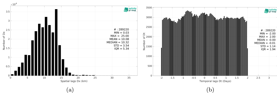
Figure 5: Histograms of the spatial (a) and temporal (b) lags between the location/time of the TSG (CSIC-UTM) measurement and the date of the corresponding SMOS SSS L3 v8 - 18 Days (CATDS-CEC-LOCEAN) SSS pixel.
