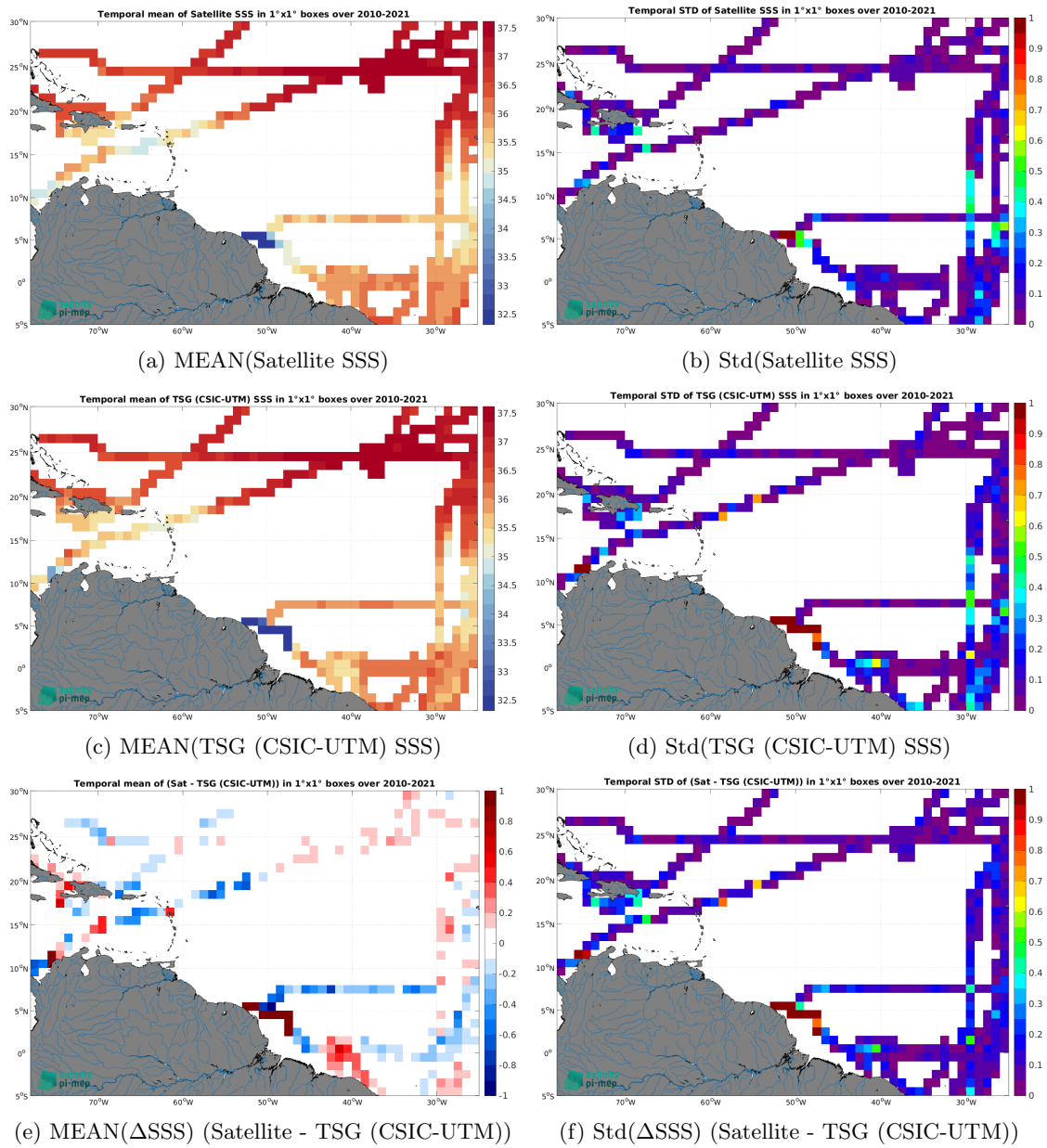
Figure 6: Temporal mean (left) and Std (right) of SSS from SMOS SSS L3 v8 - 18 Days (CATDS-CEC-LOCEAN) (top), TSG (CSIC-UTM) (middle), and of \Delta SSS (Satellite - TSG (CSIC-UTM)). Only match-up pairs are used to generate these maps.
