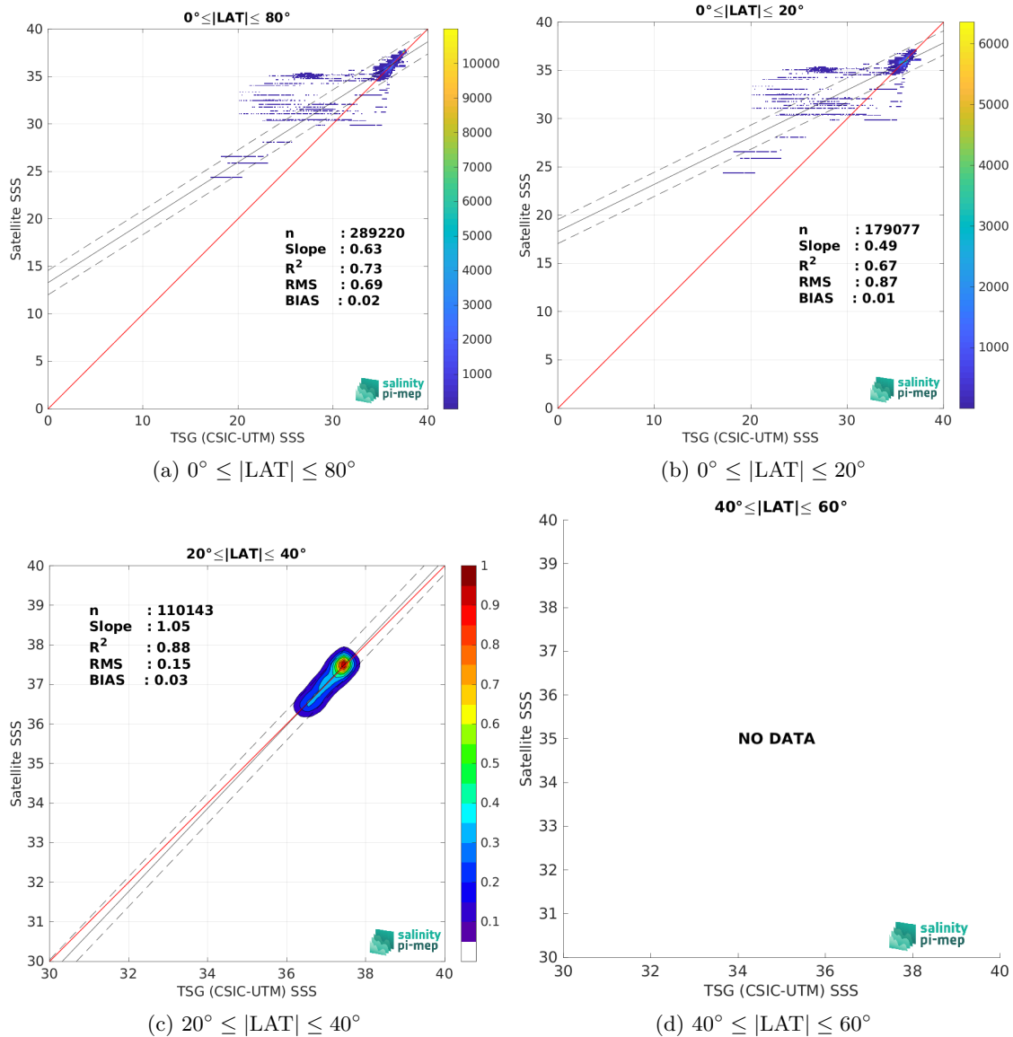
Figure 9: Contour maps of the concentration of SMOS SSS L3 v8 - 18 Days (CATDS-CEC-LOCEAN) SSS (y-axis) versus TSG (CSIC-UTM) SSS (x-axis) at match-up pairs for different latitude bands. For each plot, the red line shows x=y . The black thin and dashed lines indicate a linear fit through the data cloud and the \pm 95\% confidence levels, respectively. The number match-up pairs n , the slope and R^2 coefficient of the linear fit, the root mean square (RMS) and the mean bias between satellite and in situ data are indicated for each latitude band in each plots.
