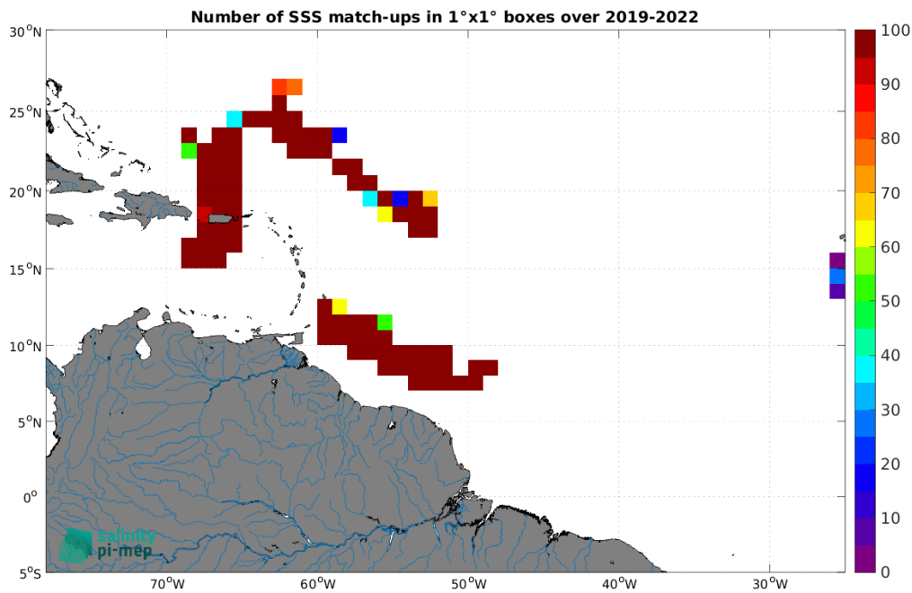
Figure 4: Number of SSS match-ups between Saildrone SSS and the SMOS SSS L3 v8 - 18 Days (CATDS-CEC-LOCEAN) SSS product for the Amazon and Orinoco river plumes Pi-MEP region over 1^\circ \times 1^\circ boxes and for the full satellite product period.
