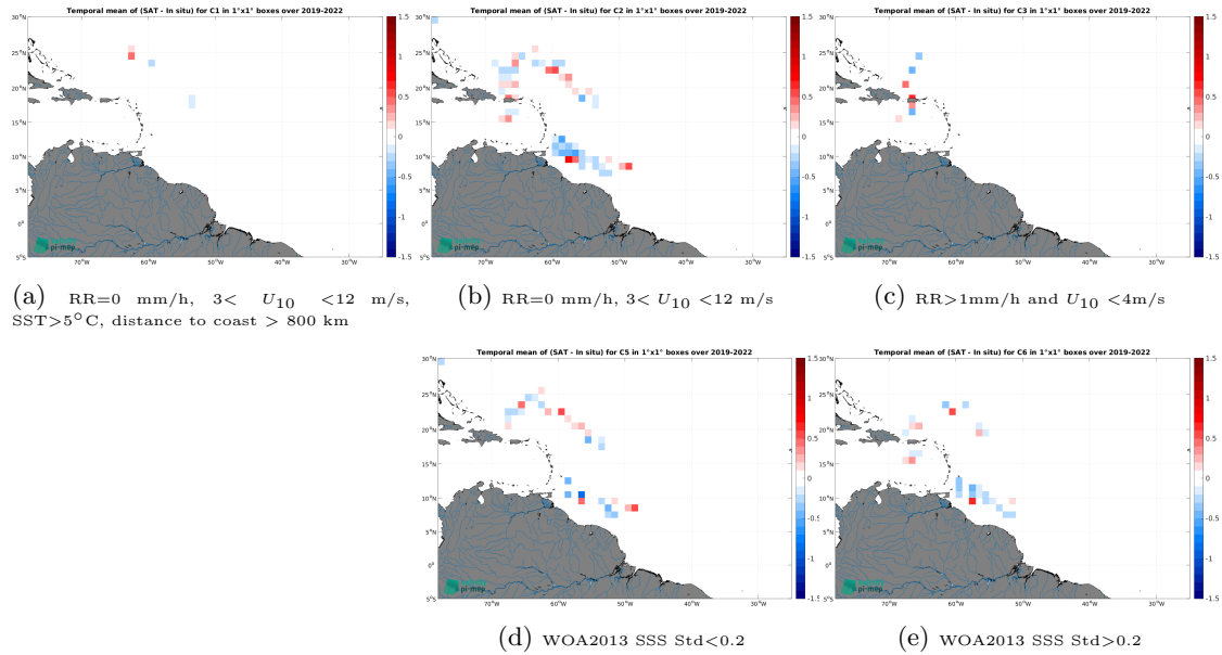
Figure 12: Temporal mean gridded over spatial boxes of size 1^\circ \times 1^\circ of \Delta SSS (SMOS SSS L3 v8 - 18 Days (CATDS-CEC-LOCEAN) - Sairdrone) for 5 different subdatasets corresponding to:RR=0 mm/h, 3 < U_{10} < 12 m/s, SST >5^\circ\text{C} , distance to coast > 800 km (a), RR=0 mm/h, 3 < U_{10} < 12 m/s (b), RR >1 mm/h and U_{10} < 4 m/s (c), WOA2013 SSS Std <0.2 (d), WOA2013 SSS Std >0.2 (e).
