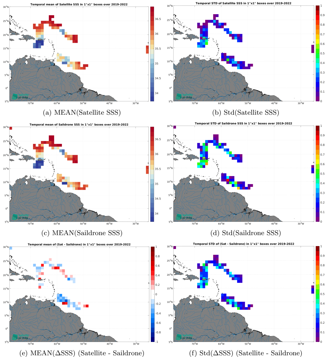
Figure 6: Temporal mean (left) and Std (right) of SSS from SMOS SSS L3 v8 - 18 Days (CATDS-CEC-LOCEAN) (top), Saildrone (middle), and of \Delta SSS (Satellite - Saildrone). Only match-up pairs are used to generate these maps.
