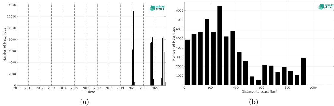
Figure 1: Number of match-ups between Saildrone and SMOS SSS L3 v8 - 18 Days (CATDS-CEC-LOCEAN) SSS as a function of time (a) and as function of the distance to coast (b) over the Amazon and Orinoco river plumes Pi-MEP region and for the full satellite product period.
