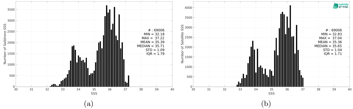
Figure 2: Histograms of SSS from Saildrone (a) and SMOS SSS L3 v8 - 18 Days (CATDS-CEC-LOCEAN) (b) considering all match-up pairs per bins of 0.1 over the Amazon and Orinoco river plumes Pi-MEP region and for the full satellite product period.
