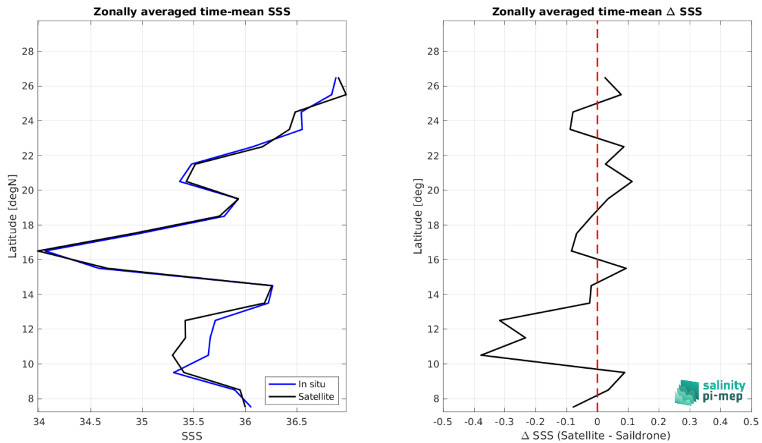
Figure 8: Left panel: Zonal mean SSS from SMOS SSS L3 v8 - 18 Days (CATDS-CEC-LOCEAN) satellite product (black) and from Sairdron (blue). Right panel: Zonal mean of \Delta SSS (Satellite - Sairdron) for all the collected Pi-MEP match-up pairs estimated over the full satellite product period.
