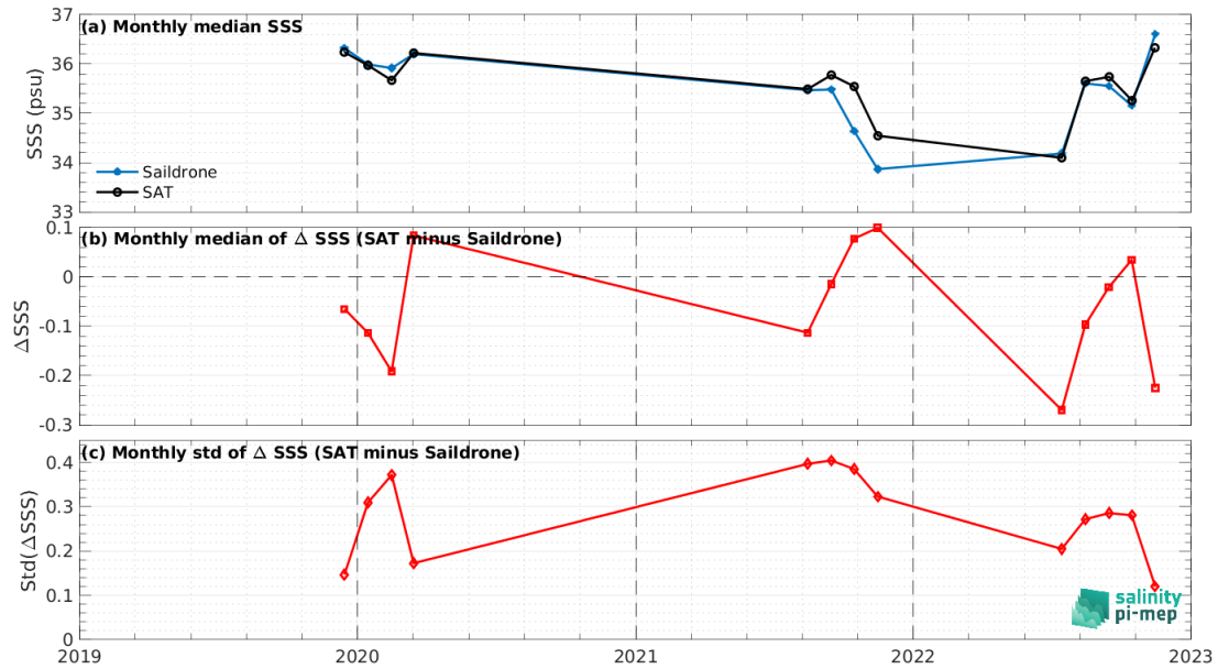
Figure 7: Time series of the monthly median SSS (top), median of \Delta SSS (Satellite - Sairdrone) and Std of \Delta SSS (Satellite - Sairdrone) over the Amazon and Orinoco river plumes Pi-MEP region considering all match-ups collected by the Pi-MEP.
