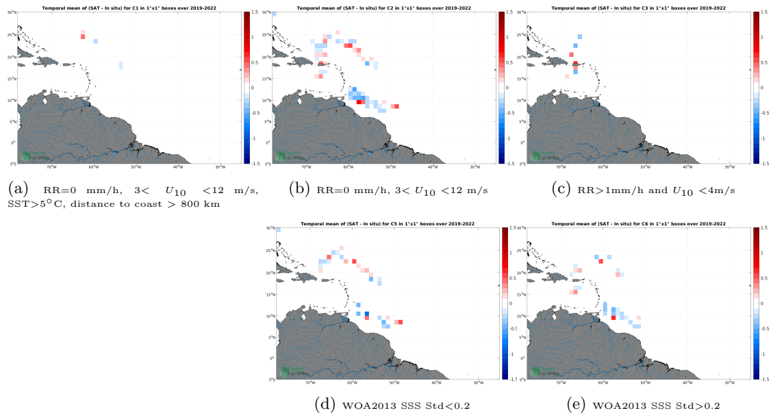
Figure 12: Temporal mean gridded over spatial boxes of size 1^\circ \times 1^\circ of \Delta SSS (SMOS SSS L3 v8 - 18 Days (CATDS-CECOS-LOCEAN) - Saildrone) for 5 different subdatasets corresponding to:RR=0 mm/h, 3 < U_{10} < 12 m/s, SST >5^\circ C, distance to coast > 800 km (a), RR=0 mm/h, 3 < U_{10} < 12 m/s (b), RR >1 mm/h and U_{10} < 4 m/s (c), WOA2013 SSS Std <0.2 (d), WOA2013 SSS Std >0.2 (e).
