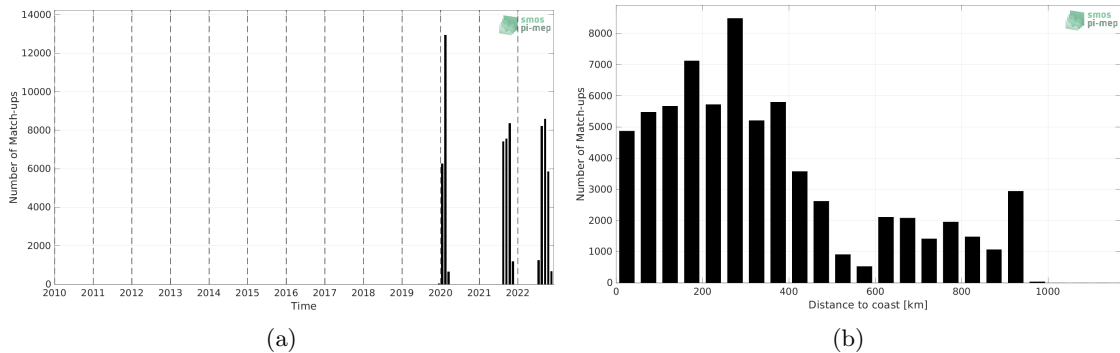
Figure 1: Number of match-ups between Saildrone and SMOS SSS L3 v8 - 18 Days (CATDS-CECOS-LOCEAN) SSS as a function of time (a) and as function of the distance to coast (b) over the Amazon and Orinoco river plumes Pi-MEP region and for the full satellite product period.
