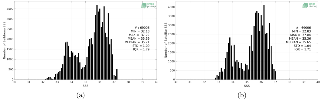
Figure 2: Histograms of SSS from Saildrone (a) and SMOS SSS L3 v8 - 18 Days (CATDS-CECOS-LOCEAN) (b) considering all match-up pairs per bins of 0.1 over the Amazon and Orinoco river plumes Pi-MEP region and for the full satellite product period.
