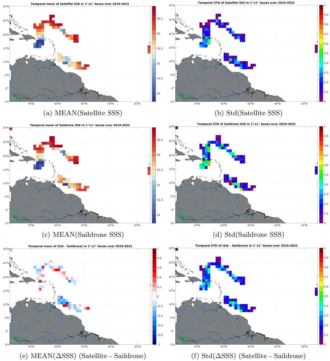
Figure 6: Temporal mean (left) and Std (right) of SSS from SMOS SSS L3 v8 - 18 Days (CATDS-CECOS-LOCEAN) (top), Saildrone (middle), and of \Delta SSS (Satellite - Saildrone). Only match-pairs are used to generate these maps.
