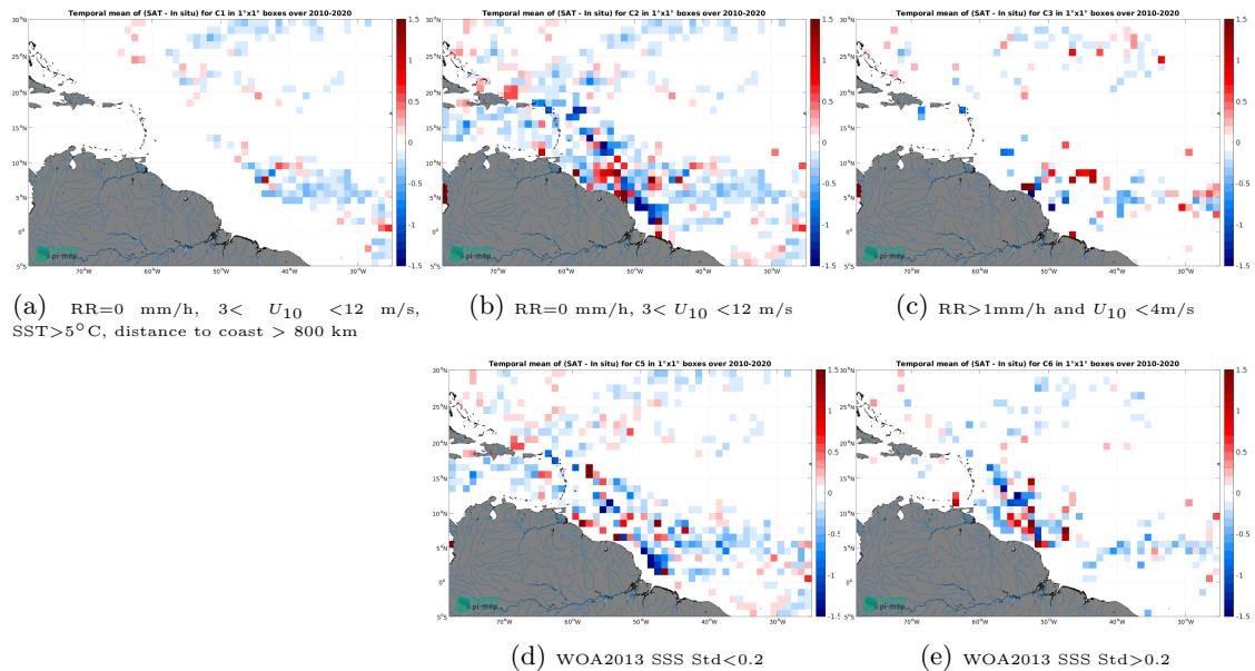
Figure 11: Temporal mean gridded over spatial boxes of size 1^\circ \times 1^\circ of \Delta\text{SSS} (SMOS SSS L3 v8 - 18 Days (CATDS-CEC-LOCEAN) - Surface drifters) for 5 different subdatasets corresponding to:RR=0 mm/h, 3 < U_{10} < 12 m/s, SST >5^\circ\text{C} , distance to coast > 800 km (a), RR=0 mm/h, 3 < U_{10} < 12 m/s (b), RR >1 mm/h and U_{10} < 4 m/s (c), WOA2013 SSS Std <0.2 (d), WOA2013 SSS Std >0.2 (e).
