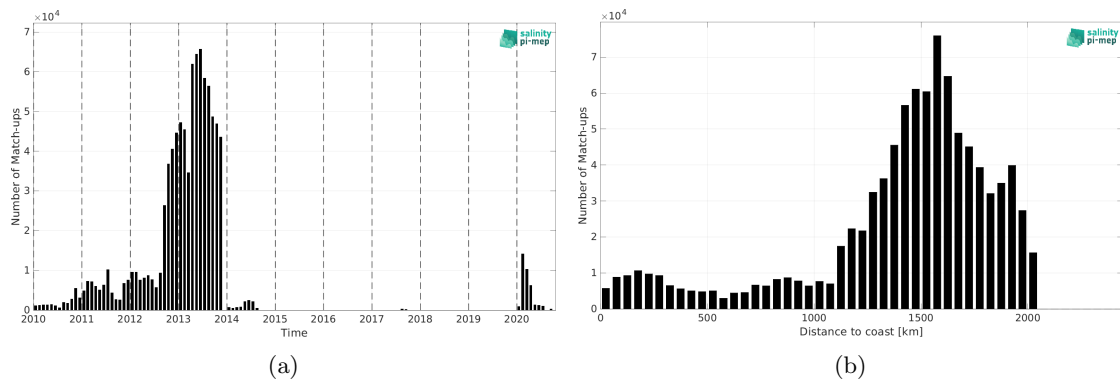
Figure 1: Number of match-ups between Surface drifters and SMOS SSS L3 v8 - 18 Days (CATDS-CEC-LOCEAN) SSS as a function of time (a) and as function of the distance to coast (b) over the Amazon and Orinoco river plumes Pi-MEP region and for the full satellite product period.
