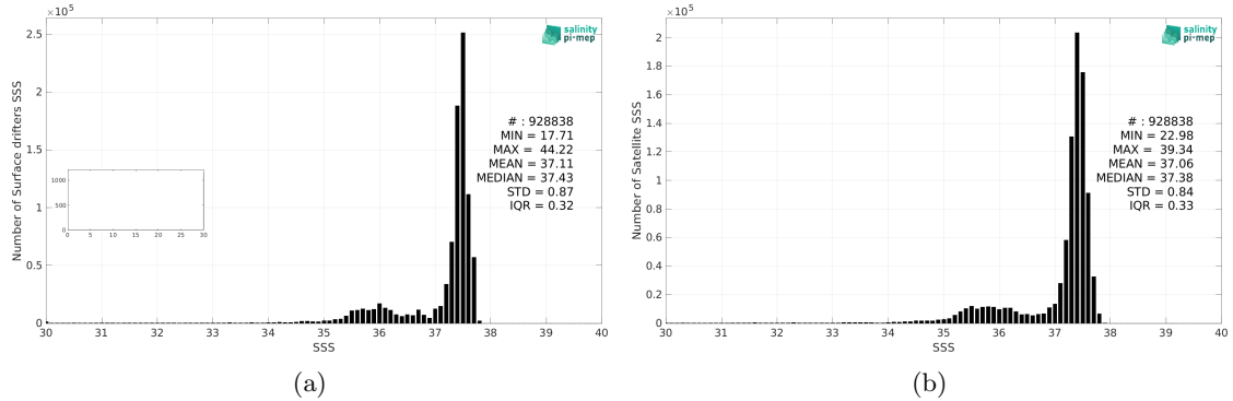
Figure 2: Histograms of SSS from Surface drifters (a) and SMOS SSS L3 v8 - 18 Days (CATDS-CEC-LOCEAN) (b) considering all match-up pairs per bins of 0.1 over the Amazon and Orinoco river plumes Pi-MEP region and for the full satellite product period.
