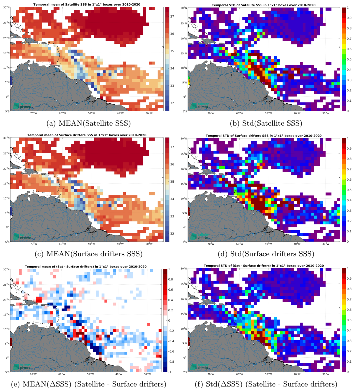
Figure 5: Temporal mean (left) and Std (right) of SSS from SMOS SSS L3 v8 - 18 Days (CATDS-CEC-LOCEAN) (top), Surface drifters (middle), and of \Delta SSS (Satellite - Surface drifters). Only match-up pairs are used to generate these maps.
