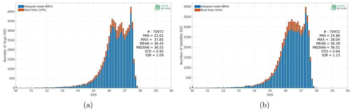
Figure 2: Histograms of SSS from Argo (a) and SMOS SSS L3 v8 - 18 Days (CATDS-CECOS-LOCEAN) (b) considering all match-up pairs per bins of 0.1 over the Amazon and Orinoco river plumes Pi-MEP region and for the full satellite product period.
