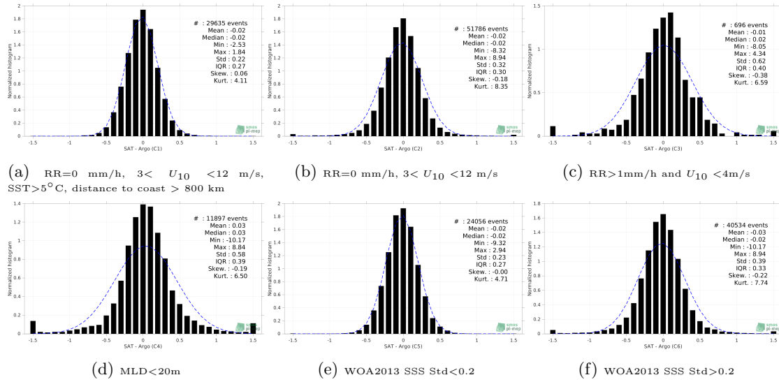
Figure 13: Normalized histogram of \Delta\text{SSS} (SMOS SSS L3 v7 - 9 Days (CATDS-CECOS-LOCEAN) - Argo) for 6 different subdatasets corresponding to: RR=0 mm/h, 3 < U_{10} < 12 m/s, SST>5°C, distance to coast > 800 km (a), RR=0 mm/h, 3 < U_{10} < 12 m/s (b), RR>1mm/h and U_{10} < 4 m/s (c), MLD<20m (d), WOA2013 SSS Std<0.2 (e), WOA2013 SSS Std>0.2 (f).
