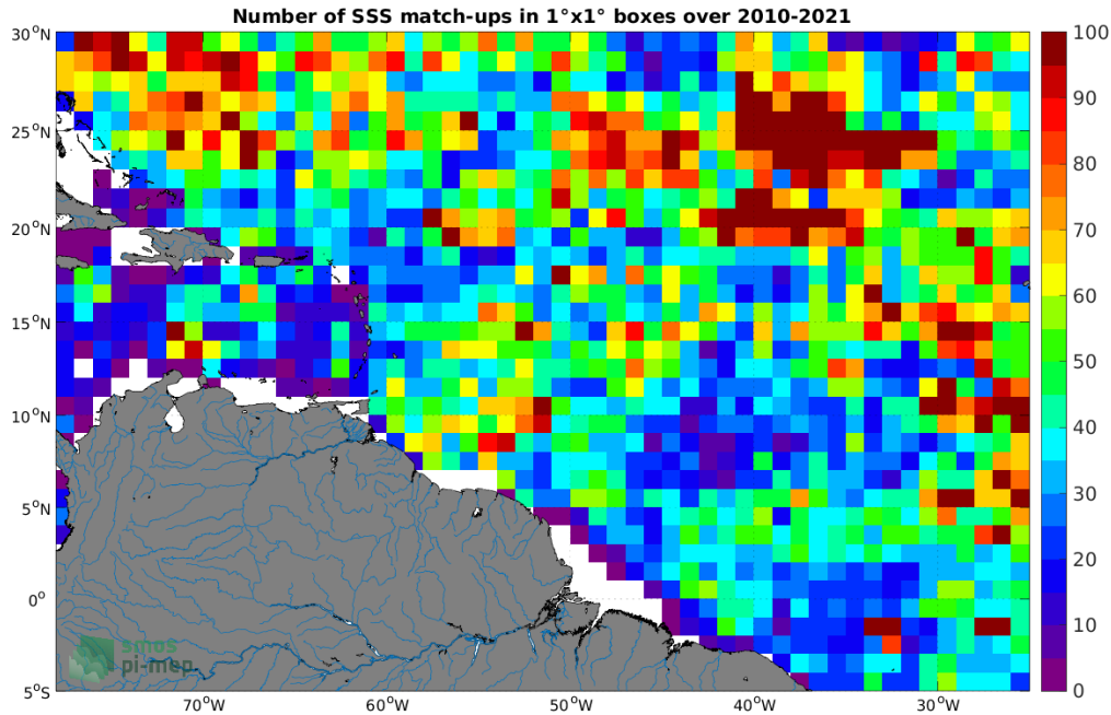
Figure 4: Number of SSS match-ups between Argo SSS and the SMOS SSS L3 v7 - 9 Days (CATDS-CECOS-LOCEAN) SSS product for the Amazon and Orinoco river plumes Pi-MEP region over 1^{\circ} \times 1^{\circ} boxes and for the full satellite product period.
