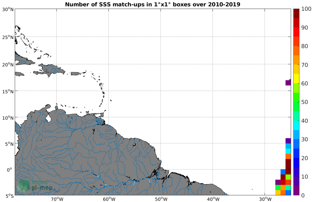
Figure 4: Number of SSS match-ups between TSG (Polarstern) SSS and the SMOS SSS L3 v5 - 9 Days (CATDS-CECOS-LOCEAN) SSS product for the Amazon and Orinoco river plumes Pi-MEP region over 1°x1° boxes and for the full satellite product period.
