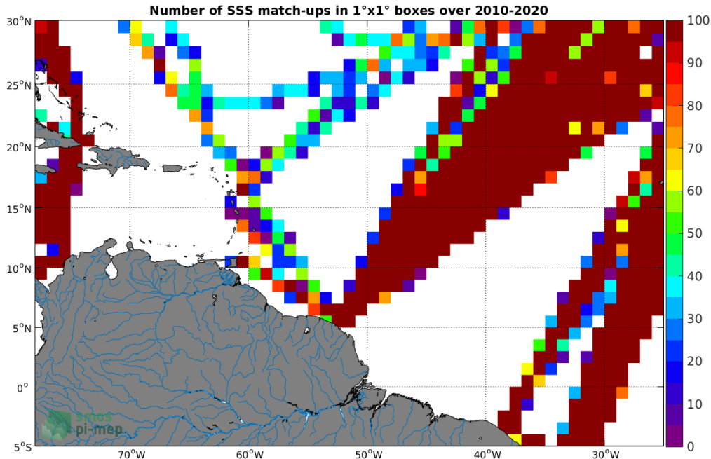
Figure 4: Number of SSS match-ups between TSG (LEGOS-DM) SSS and the SMOS SSS L3 v5 - 9 Days (CATDS-CECOS-LOCEAN) SSS product for the Amazon and Orinoco river plumes Pi-MEP region over 1^{\circ} \times 1^{\circ} boxes and for the full satellite product period.
