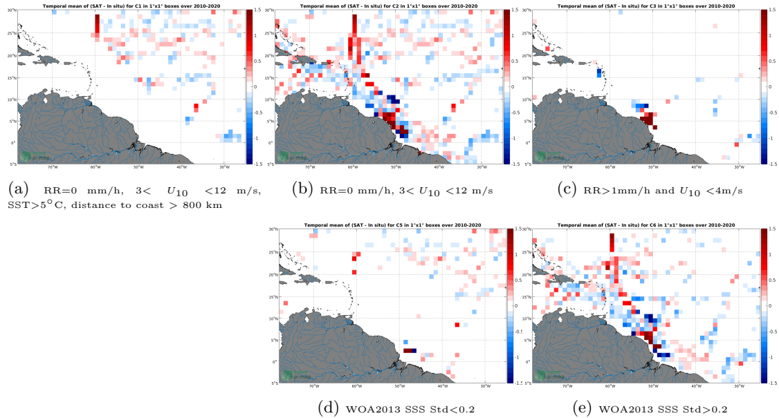
Figure 12: Temporal mean gridded over spatial boxes of size 1^\circ \times 1^\circ of \Delta SSS (SMOS SSS L3 v5 - 9 Days (CATDS-CECOS-LOCEAN) - TSG (GOSUD-Research-vessel)) for 5 different subdatasets corresponding to:RR=0 mm/h, 3 < U_{10} < 12 m/s, SST >5^\circ\text{C} , distance to coast > 800 km (a), RR=0 mm/h, 3 < U_{10} < 12 m/s (b), RR >1 mm/h and U_{10} < 4 m/s (c), WOA2013 SSS Std <0.2 (d), WOA2013 SSS Std >0.2 (e).
