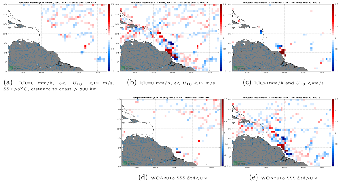
Figure 12: Temporal mean gridded over spatial boxes of size 1^{\circ}\times 1^{\circ} of \Delta SSS (SMOS SSS L3 v5 - 9 Days (CATDS-CECOS-LOCEAN) - TSG (GOSUD-Research-vessel)) for 5 different subdatasets corresponding to:RR=0 mm/h, 3 < U_{10} < 12 m/s, SST >5^{\circ}\text{C} , distance to coast > 800 km (a), RR=0 mm/h, 3 < U_{10} < 12 m/s (b), RR >1 mm/h and U_{10} < 4 m/s (c), WOA2013 SSS Std <0.2 (d), WOA2013 SSS Std >0.2 (e).
