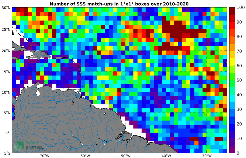
Figure 4: Number of SSS match-ups between Argo SSS and the SMOS SSS L3 v5 - 9 Days (CATDS-CECOS-LOCEAN) SSS product for the Amazon and Orinoco river plumes Pi-MEP region over 1°x1° boxes and for the full satellite product period.
