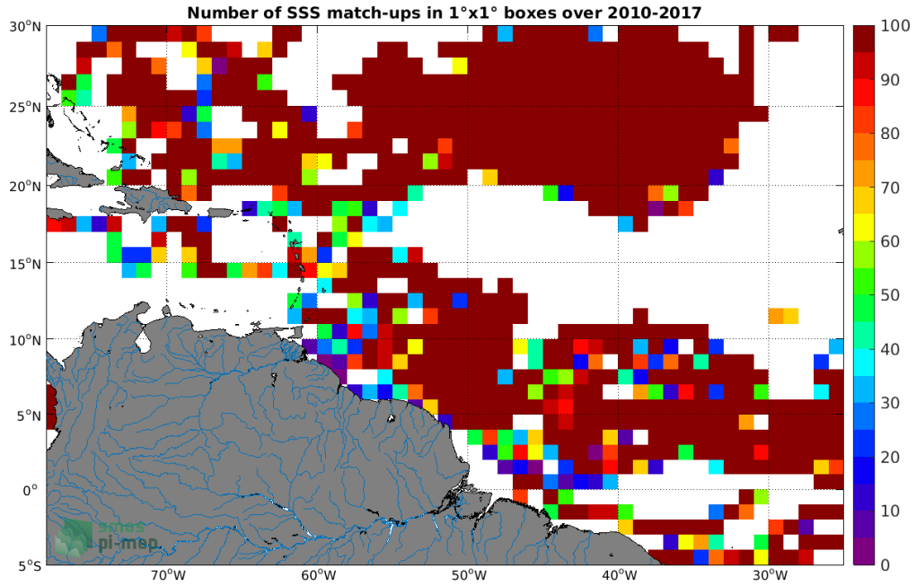
Figure 3: Number of SSS match-ups between Surface drifters SSS and the SMOS SSS L3 v5 - 18 Days (CATDS-CECOS-LOCEAN) SSS product for the Amazon and Orinoco river plumes Pi-MEP region over 1°x1° boxes and for the full satellite product period.
