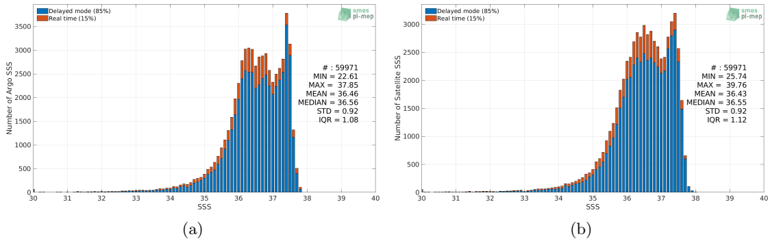
Figure 2: Histograms of SSS from Argo (a) and SMOS SSS L3 v5 - 18 Days (CATDS-CECOS-LOCEAN) (b) considering all match-up pairs per bins of 0.1 over the Amazon and Orinoco river plumes Pi-MEP region and for the full satellite product period.
