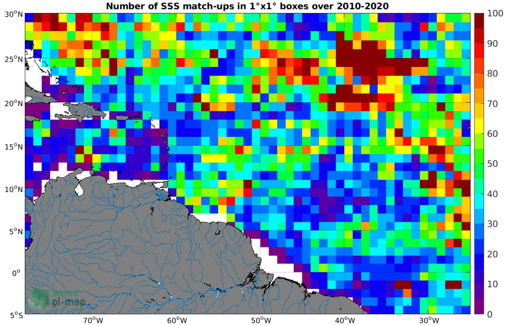
Figure 4: Number of SSS match-ups between Argo SSS and the SMOS SSS L3 v5 - 18 Days (CATDS-CECOS-LOCEAN) SSS product for the Amazon and Orinoco river plumes Pi-MEP region over 1^\circ \times 1^\circ boxes and for the full satellite product period.
