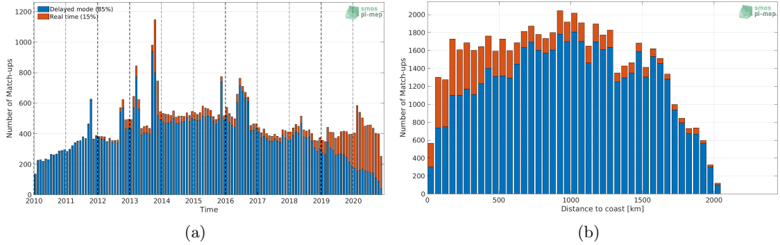
Figure 1: Number of match-ups between Argo and SMOS SSS L3 v5 - 18 Days (CATDS-CECOS-LOCEAN) SSS as a function of time (a) and as function of the distance to coast (b) over the Amazon and Orinoco river plumes Pi-MEP region and for the full satellite product period.
