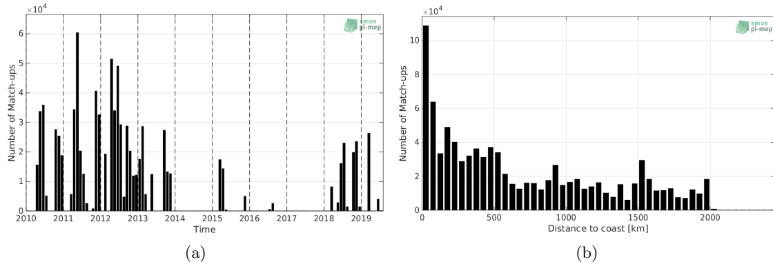
Figure 1: Number of match-ups between TSG-SAMOS and SMOS-L3-CATDS-CECOS-LOCEAN-V4-9DAYS-25KM SSS as a function of time (a) and as function of the distance to coast (b) over the Amazon and Orinoco river plumes Pi-MEP region and for the full satellite product period.
