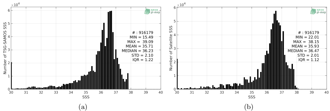
Figure 2: Histograms of SSS from TSG-SAMOS (a) and SMOS-L3-CATDS-CECOS-LOCEAN-V4-9DAYS-25KM (b) considering all match-up pairs per bins of 0.1 over the Amazon and Orinoco river plumes Pi-MEP region and for the full satellite product period.
