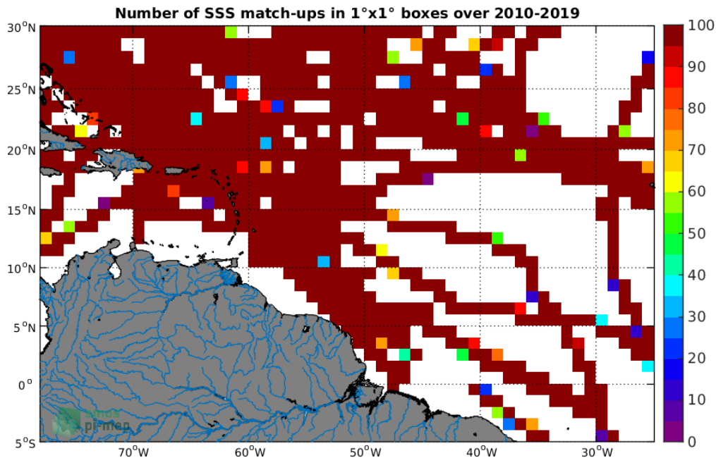
Figure 4: Number of SSS match-ups between TSG-SAMOS SSS and the SMOS-L3-CATDS-CECOS-LOCEAN-V4-9DAYS-25KM SSS product for the Amazon and Orinoco river plumes Pi-MEP region over 1^\circ \times 1^\circ boxes and for the full satellite product period.
