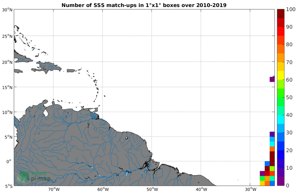
Figure 4: Number of SSS match-ups between TSG-POLARSTERN SSS and the SMOS-L3-CATDS-CECOS-LOCEAN-V4-9DAYS-25KM SSS product for the Amazon and Orinoco river plumes Pi-MEP region over 1^\circ \times 1^\circ boxes and for the full satellite product period.
