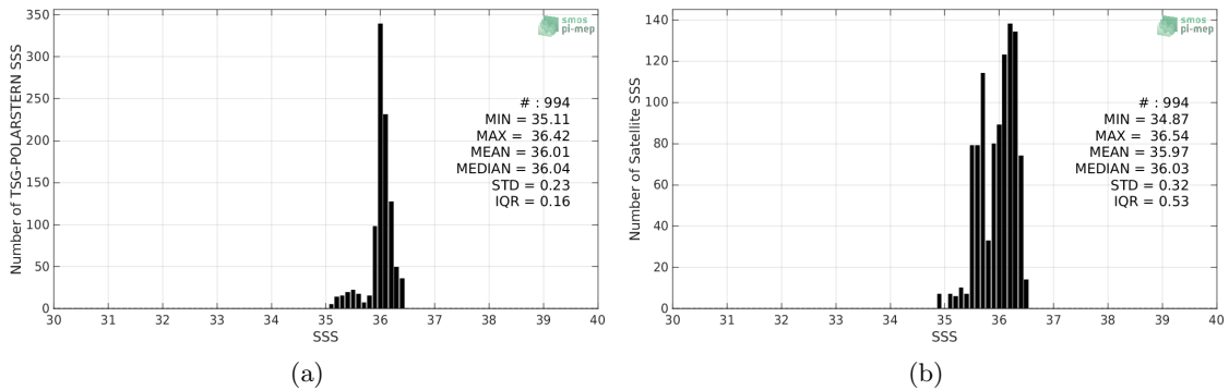
Figure 2: Histograms of SSS from TSG-POLARSTERN (a) and SMOS-L3-CATDS-CECOS-LOCEAN-V4-9DAYS-25KM (b) considering all match-up pairs per bins of 0.1 over the Amazon and Orinoco river plumes Pi-MEP region and for the full satellite product period.
