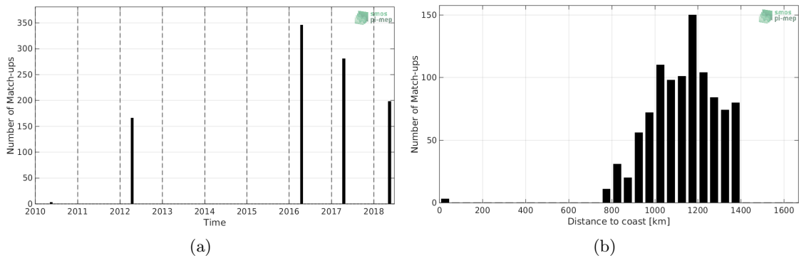
Figure 1: Number of match-ups between TSG-POLARSTERN and SMOS-L3-CATDS-CECOS-LOCEAN-V4-9DAYS-25KM SSS as a function of time (a) and as function of the distance to coast (b) over the Amazon and Orinoco river plumes Pi-MEP region and for the full satellite product period.
