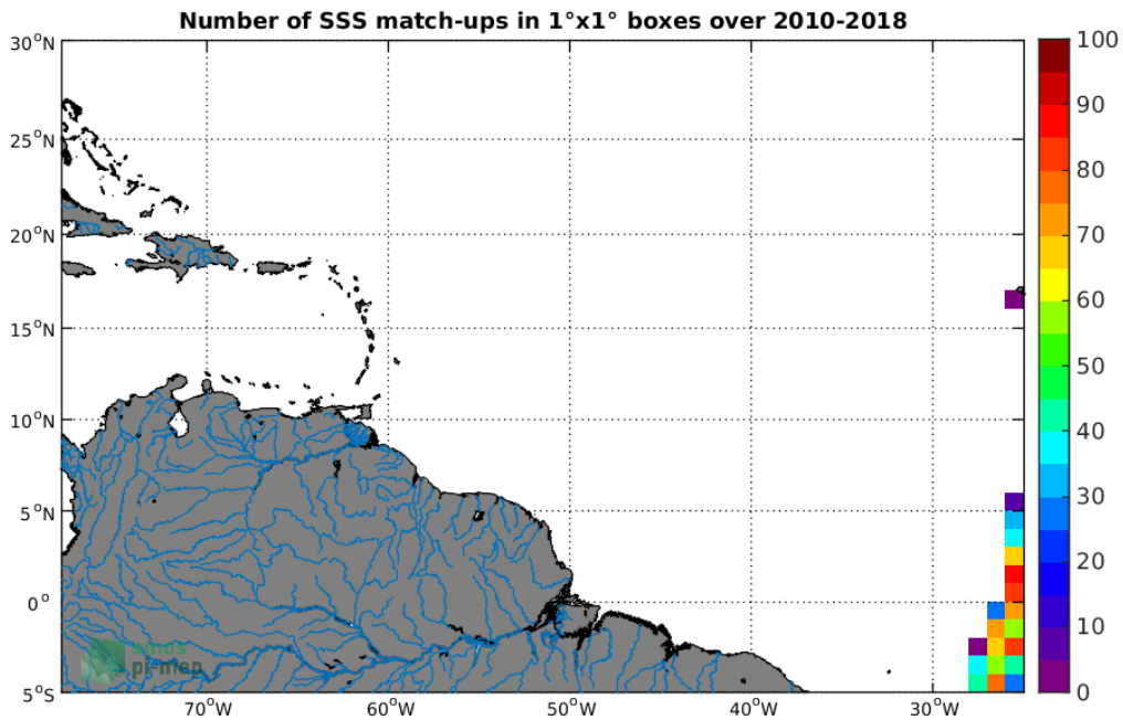
Figure 4: Number of SSS match-ups between TSG-POLARSTERN SSS and the SMOS-L3-CATDS-CECOS-LOCEAN-V4-9DAYS-25KM SSS product for the Amazon and Orinoco river plumes Pi-MEP region over 1°x1° boxes and for the full satellite product period.
