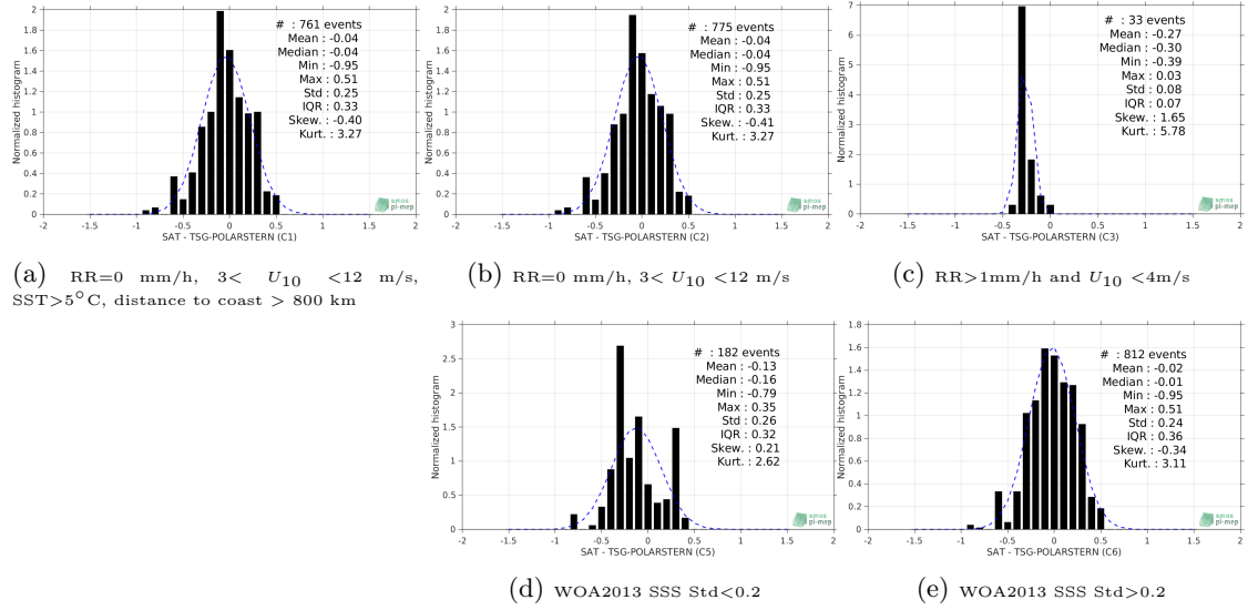
Figure 13: Normalized histogram of \Delta SSS (SMOS-L3-CATDS-CECOS-LOCEAN-V4-9DAYS-25KM - TSG-POLARSTERN) for 5 different subdatasets corresponding to: RR=0 mm/h, 3 < U_{10} < 12 m/s, SST > 5°C, distance to coast > 800 km (a), RR=0 mm/h, 3 < U_{10} < 12 m/s (b), RR > 1mm/h and U_{10} < 4 m/s (c), WOA2013 SSS Std < 0.2 (d), WOA2013 SSS Std > 0.2 (e).
