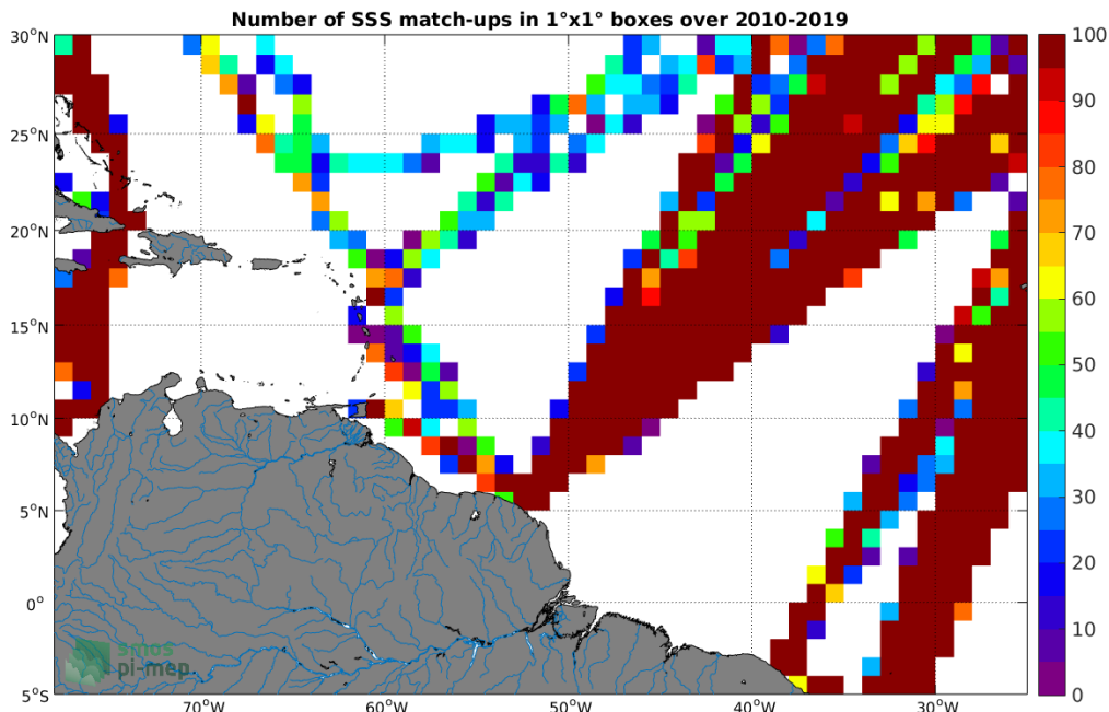
Figure 4: Number of SSS match-ups between TSG (LEGOS-DM) SSS and the SMOS SSS L3 v4 - 9 Days (CATDS-CECOS-LOCEAN) SSS product for the Amazon and Orinoco river plumes Pi-MEP region over 1^\circ \times 1^\circ boxes and for the full satellite product period.
