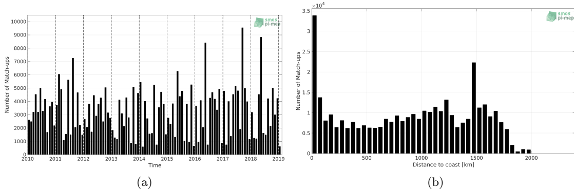
Figure 1: Number of match-ups between TSG (LEGOS-DM) and SMOS SSS L3 v4 - 9 Days (CATDS-CECOS-LOCEAN) SSS as a function of time (a) and as function of the distance to coast (b) over the Amazon and Orinoco river plumes Pi-MEP region and for the full satellite product period.
