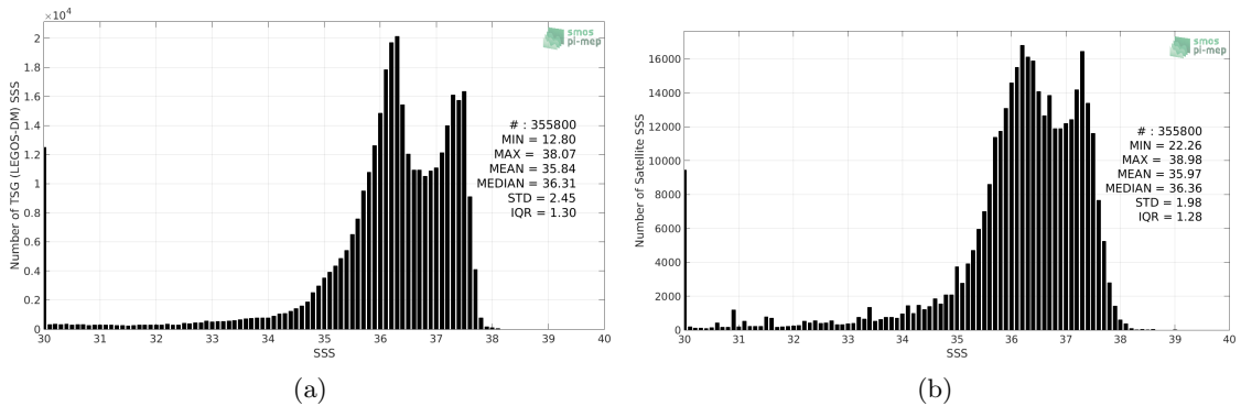
Figure 2: Histograms of SSS from TSG (LEGOS-DM) (a) and SMOS SSS L3 v4 - 9 Days (CATDS-CECOS-LOCEAN) (b) considering all match-up pairs per bins of 0.1 over the Amazon and Orinoco river plumes Pi-MEP region and for the full satellite product period.
