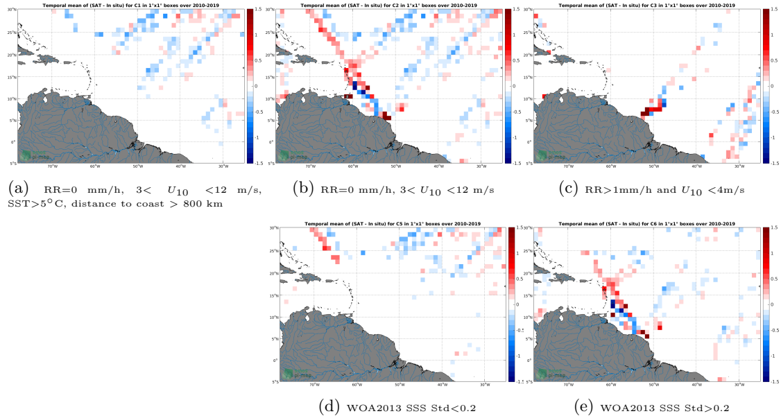
Figure 12: Temporal mean gridded over spatial boxes of size 1^{\circ}\times 1^{\circ} of \Delta\text{SSS} (SMOS SSS L3 v4 - 9 Days (CATDS-CECOS-LOCEAN) - TSG (LEGOS-DM)) for 5 different subdatasets corresponding to:RR=0 mm/h, 3 < U_{10} < 12 m/s, SST >5^{\circ}\text{C} , distance to coast > 800 km (a), RR=0 mm/h, 3 < U_{10} < 12 m/s (b), RR >1 mm/h and U_{10} < 4 m/s (c), WOA2013 SSS Std <0.2 (d), WOA2013 SSS Std >0.2 (e).
