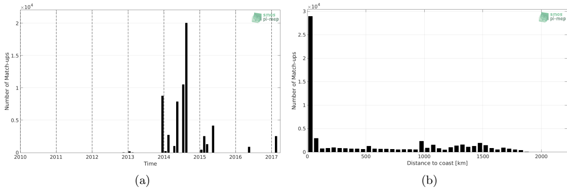
Figure 1: Number of match-ups between TSG (GOSUD-Sailing-ship) and SMOS SSS L3 v4 - 9 Days (CATDS-CECOS-LOCEAN) SSS as a function of time (a) and as function of the distance to coast (b) over the Amazon and Orinoco river plumes Pi-MEP region and for the full satellite product period.
