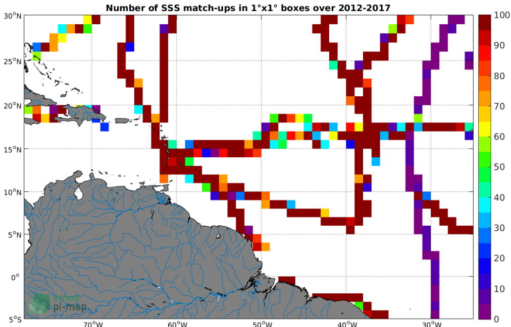
Figure 4: Number of SSS match-ups between TSG (GOSUD-Sailing-ship) SSS and the SMOS SSS L3 v4 - 9 Days (CATDS-CECOS-LOCEAN) SSS product for the Amazon and Orinoco river plumes Pi-MEP region over 1^\circ \times 1^\circ boxes and for the full satellite product period.
