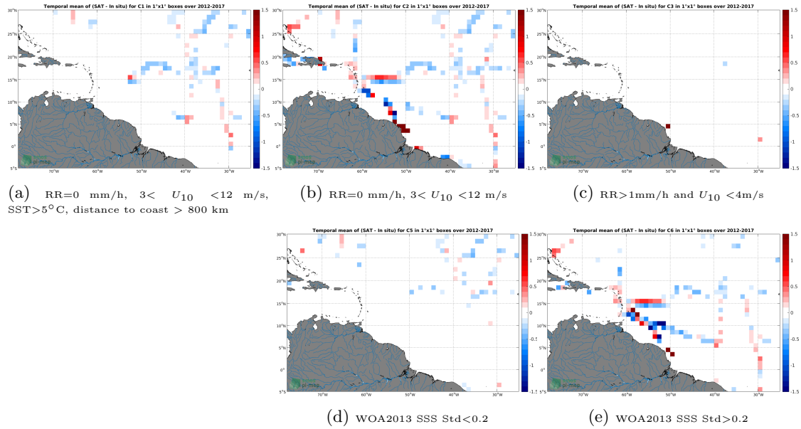
Figure 12: Temporal mean gridded over spatial boxes of size 1^{\circ}\times 1^{\circ} of \Delta SSS (SMOS SSS L3 v4 - 9 Days (CATDS-CECOS-LOCEAN) - TSG (GOSUD-Sailing-ship)) for 5 different subdatasets corresponding to:RR=0 mm/h, 3 < U_{10} < 12 m/s, SST >5^{\circ}\text{C} , distance to coast > 800 km (a), RR=0 mm/h, 3 < U_{10} < 12 m/s (b), RR >1 mm/h and U_{10} < 4 m/s (c), WOA2013 SSS Std <0.2 (d), WOA2013 SSS Std >0.2 (e).
