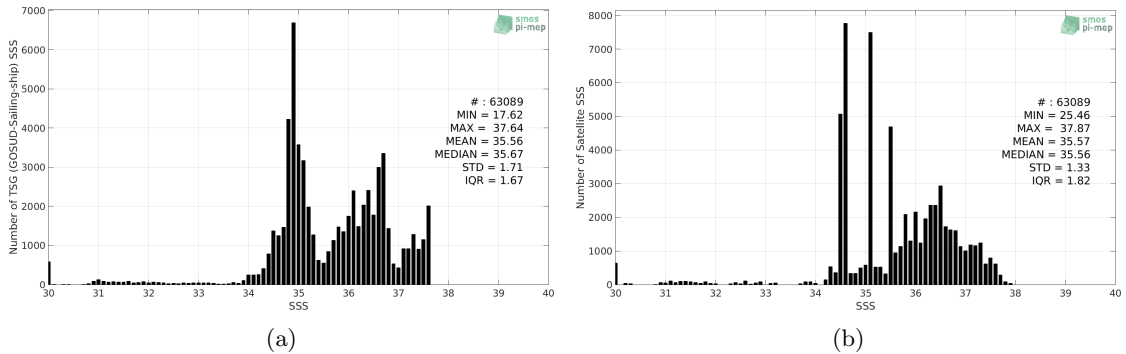
Figure 2: Histograms of SSS from TSG (GOSUD-Sailing-ship) (a) and SMOS SSS L3 v4 - 9 Days (CATDS-CECOS-LOCEAN) (b) considering all match-up pairs per bins of 0.1 over the Amazon and Orinoco river plumes Pi-MEP region and for the full satellite product period.
