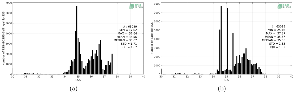
Figure 2: Histograms of SSS from TSG-GOSUD-Sailing-ship (a) and SMOS-L3-CATDS-CECOS-LOCEAN-V4-9DAYS-25KM (b) considering all match-up pairs per bins of 0.1 over the Amazon and Orinoco river plumes Pi-MEP region and for the full satellite product period.
