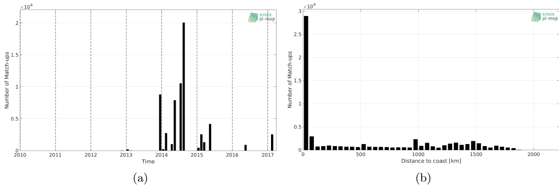
Figure 1: Number of match-ups between TSG-GOSUD-Sailing-ship and SMOS-L3-CATDS-CECOS-LOCEAN-V4-9DAYS-25KM SSS as a function of time (a) and as function of the distance to coast (b) over the Amazon and Orinoco river plumes Pi-MEP region and for the full satellite product period.
