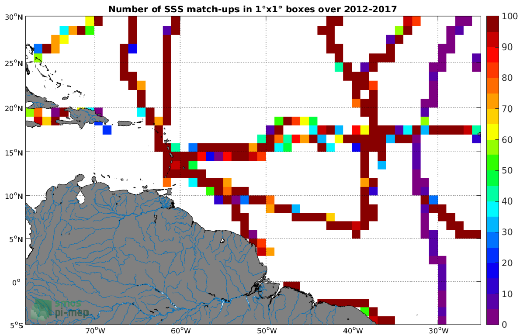
Figure 4: Number of SSS match-ups between TSG-GOSUD-Sailing-ship SSS and the SMOS-L3-CATDS-CECOS-LOCEAN-V4-9DAYS-25KM SSS product for the Amazon and Orinoco river plumes Pi-MEP region over 1^\circ \times 1^\circ boxes and for the full satellite product period.
