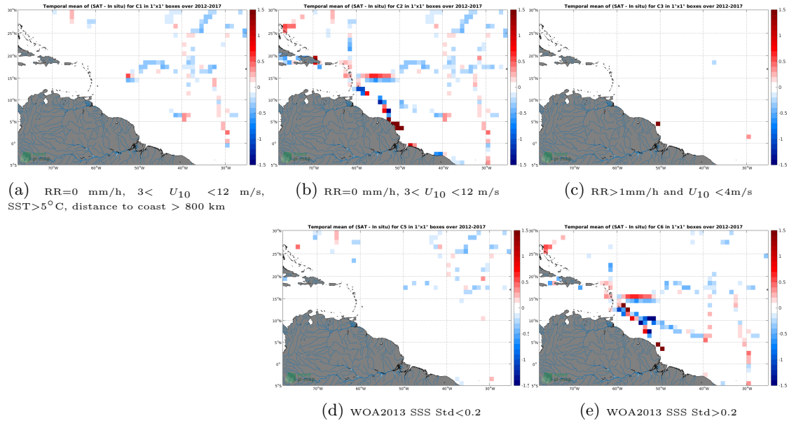
Figure 12: Temporal mean gridded over spatial boxes of size 1^{\circ}\times 1^{\circ} of \Delta SSS (SMOS-L3-CATDS-CECOS-LOCEAN-V4-9DAYS-25KM - TSG-GOSUD-Sailing-ship) for 5 different subdatasets corresponding to:RR=0 mm/h, 3 < U_{10} < 12 m/s, SST >5^{\circ}\text{C} , distance to coast > 800 km (a), RR=0 mm/h, 3 < U_{10} < 12 m/s (b), RR >1 mm/h and U_{10} < 4 m/s (c), WOA2013 SSS Std <0.2 (d), WOA2013 SSS Std >0.2 (e).
