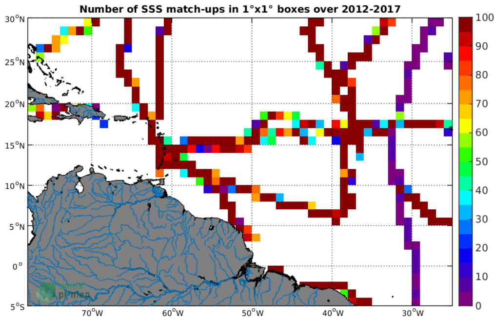
Figure 4: Number of SSS match-ups between TSG-GOSUD-Sailing-ship SSS and the SMOS-L3-CATDS-CECOS-LOCEAN-V4-9DAYS-25KM SSS product for the Amazon and Orinoco river plumes Pi-MEP region over 1°x1° boxes and for the full satellite product period.
