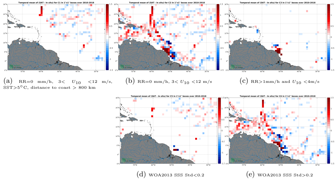
Figure 12: Temporal mean gridded over spatial boxes of size 1^{\circ}\times 1^{\circ} of \Delta SSS (SMOS-L3-CATDS-CECOS-LOCEAN-V4-9DAYS-25KM - TSG-GOSUD-Research-vessel) for 5 different subdatasets corresponding to:RR=0 mm/h, 3 < U_{10} < 12 m/s, SST >5^{\circ}\text{C} , distance to coast > 800 km (a), RR=0 mm/h, 3 < U_{10} < 12 m/s (b), RR >1 mm/h and U_{10} < 4 m/s (c), WOA2013 SSS Std <0.2 (d), WOA2013 SSS Std >0.2 (e).
