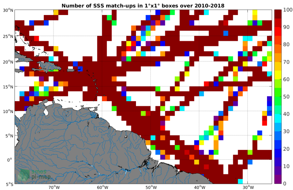
Figure 4: Number of SSS match-ups between TSG-GOSUD-Research-vessel SSS and the SMOS-L3-CATDS-CECOS-LOCEAN-V4-9DAYS-25KM SSS product for the Amazon and Orinoco river plumes Pi-MEP region over 1^\circ \times 1^\circ boxes and for the full satellite product period.
