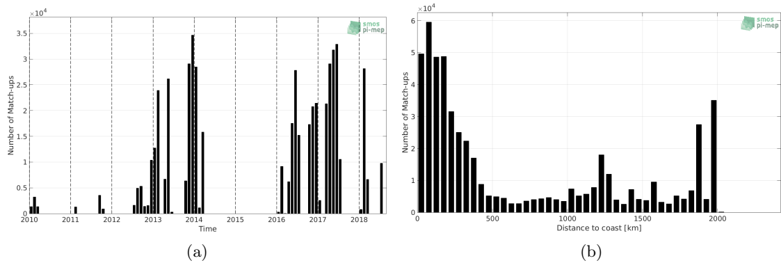
Figure 1: Number of match-ups between TSG-GOSUD-Research-vessel and SMOS-L3-CATDS-CECOS-LOCEAN-V4-9DAYS-25KM SSS as a function of time (a) and as function of the distance to coast (b) over the Amazon and Orinoco river plumes Pi-MEP region and for the full satellite product period.
