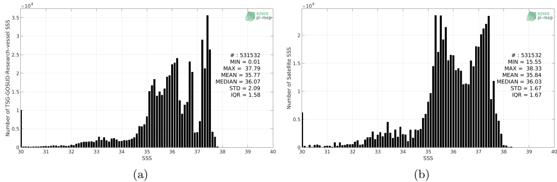
Figure 2: Histograms of SSS from TSG-GOSUD-Research-vessel (a) and SMOS-L3-CATDS-CECOS-LOCEAN-V4-9DAYS-25KM (b) considering all match-up pairs per bins of 0.1 over the Amazon and Orinoco river plumes Pi-MEP region and for the full satellite product period.
