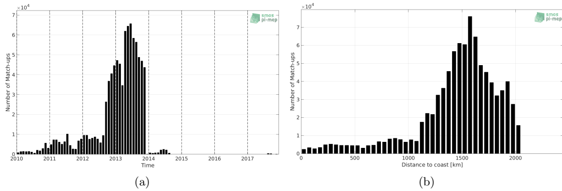
Figure 1: Number of match-ups between Surface drifters and SMOS SSS L3 v4 - 9 Days (CATDS-CECOS-LOCEAN) SSS as a function of time (a) and as function of the distance to coast (b) over the Amazon and Orinoco river plumes Pi-MEP region and for the full satellite product period.
