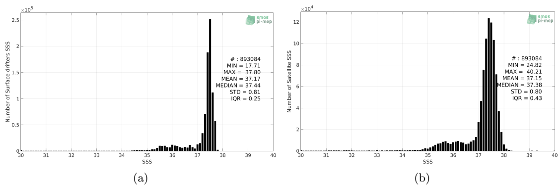
Figure 2: Histograms of SSS from Surface drifters (a) and SMOS SSS L3 v4 - 9 Days (CATDS-CECOS-LOCEAN) (b) considering all match-up pairs per bins of 0.1 over the Amazon and Orinoco river plumes Pi-MEP region and for the full satellite product period.
