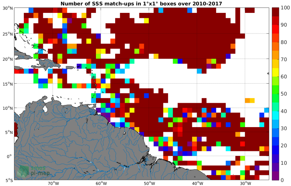
Figure 3: Number of SSS match-ups between Surface drifters SSS and the SMOS SSS L3 v4 - 9 Days (CATDS-CECOS-LOCEAN) SSS product for the Amazon and Orinoco river plumes Pi-MEP region over 1°x1° boxes and for the full satellite product period.
