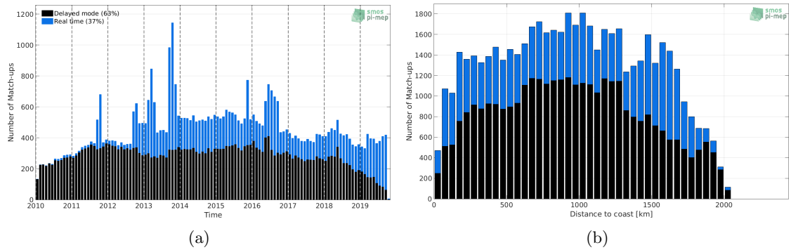
Figure 1: Number of match-ups between Argo and SMOS-L3-CATDS-CECOS-LOCEAN-V4-9DAYS-25KM SSS as a function of time (a) and as function of the distance to coast (b) over the Amazon and Orinoco river plumes Pi-MEP region and for the full satellite product period.
