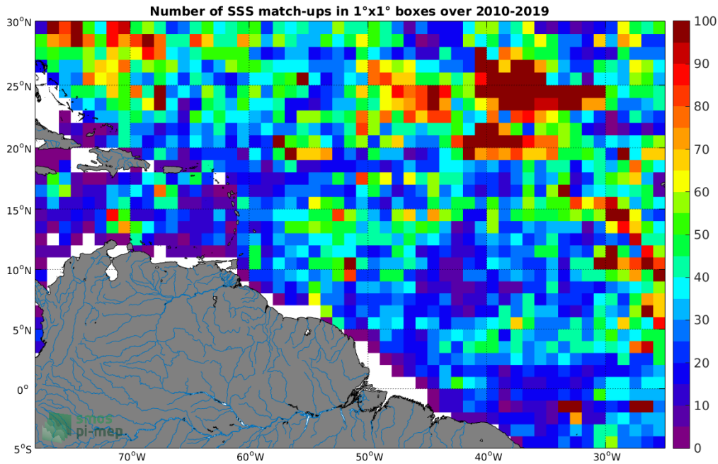
Figure 4: Number of SSS match-ups between Argo SSS and the SMOS-L3-CATDS-CECOS-LOCEAN-V4-9DAYS-25KM SSS product for the Amazon and Orinoco river plumes Pi-MEP region over 1°x1° boxes and for the full satellite product period.
