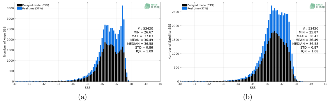
Figure 2: Histograms of SSS from Argo (a) and SMOS-L3-CATDS-CECOS-LOCEAN-V4-9DAYS-25KM (b) considering all match-up pairs per bins of 0.1 over the Amazon and Orinoco river plumes Pi-MEP region and for the full satellite product period.
