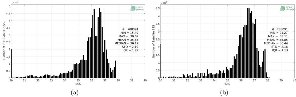
Figure 2: Histograms of SSS from TSG-SAMOS (a) and SMOS-L3-CATDS-CECOS-LOCEAN-V3-9DAYS-25KM (b) considering all match-up pairs per bins of 0.1 over the Amazon and Orinoco river plumes Pi-MEP region and for the full satellite product period.
