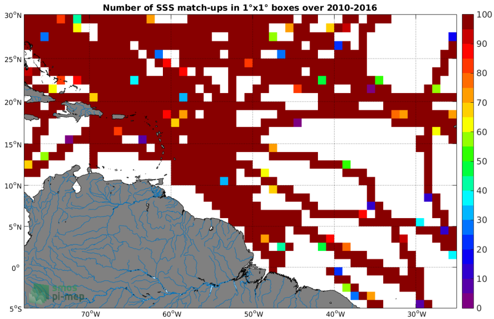
Figure 4: Number of SSS match-ups between TSG-SAMOS SSS and the SMOS-L3-CATDS-CECOS-LOCEAN-V3-9DAYS-25KM SSS product for the Amazon and Orinoco river plumes Pi-MEP region over 1^\circ \times 1^\circ boxes and for the full satellite product period.
