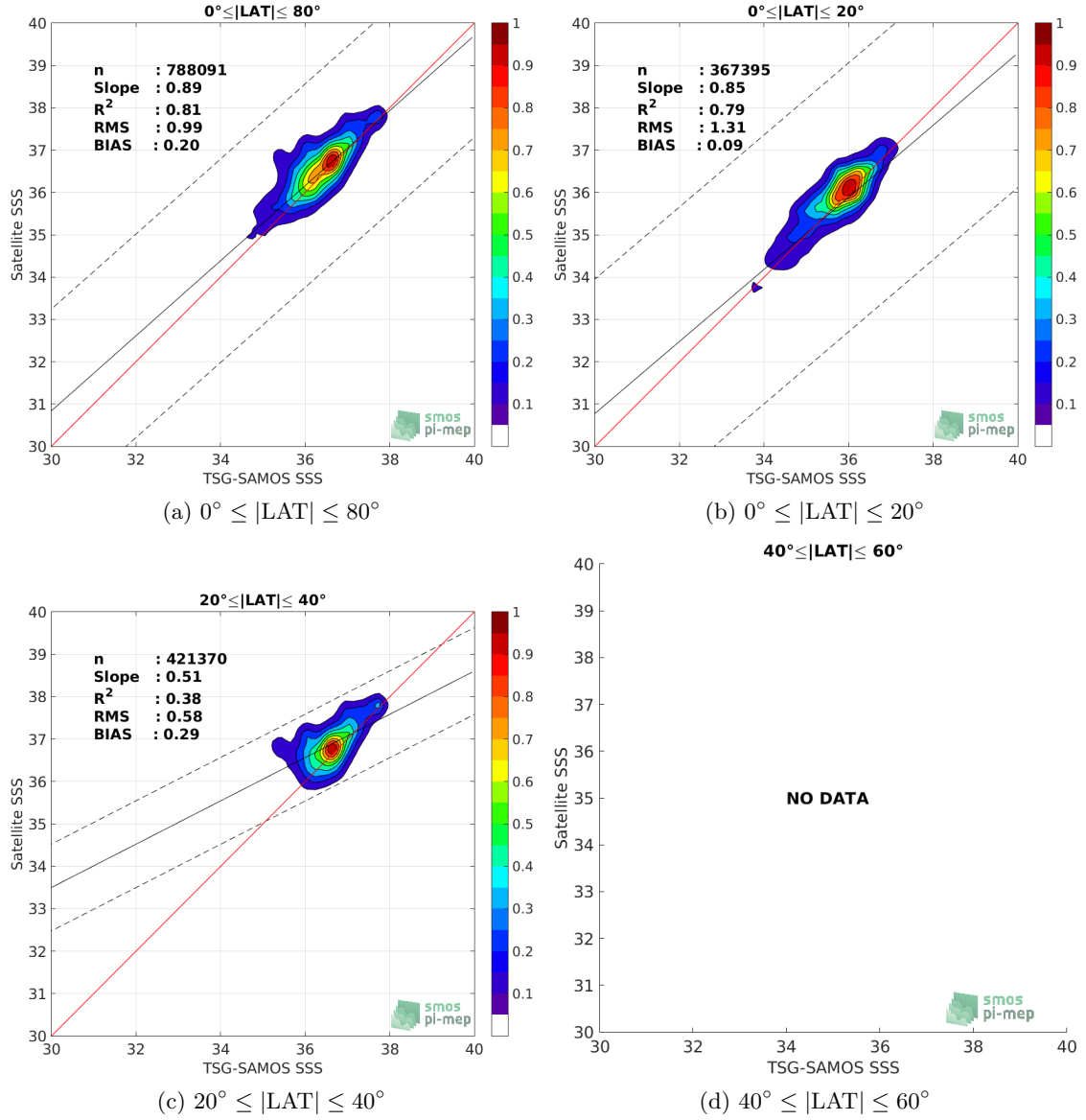
Figure 9: Contour maps of the concentration of SMOS-L3-CATDS-CECOS-LOCEAN-V3-9DAYS-25KM SSS (y-axis) versus TSG-SAMOS SSS (x-axis) at match-up pairs for different latitude bands. For each plot, the red line shows x=y . The black thin and dashed lines indicate a linear fit through the data cloud and the \pm 95\% confidence levels, respectively. The number of match-up pairs n , the slope and R^2 coefficient of the linear fit, the root mean square (RMS) and the mean bias between satellite and in situ data are indicated for each latitude band in each plot.
