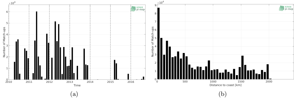
Figure 1: Number of match-ups between TSG-SAMOS and SMOS-L3-CATDS-CECOS-LOCEAN-V3-9DAYS-25KM SSS as a function of time (a) and as function of the distance to coast (b) over the Amazon and Orinoco river plumes Pi-MEP region and for the full satellite product period.
