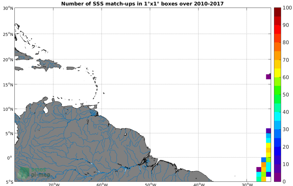
Figure 4: Number of SSS match-ups between TSG-POLARSTERN SSS and the SMOS-L3-CATDS-CECOS-LOCEAN-V3-9DAYS-25KM SSS product for the Amazon and Orinoco river plumes Pi-MEP region over 1^\circ \times 1^\circ boxes and for the full satellite product period.
