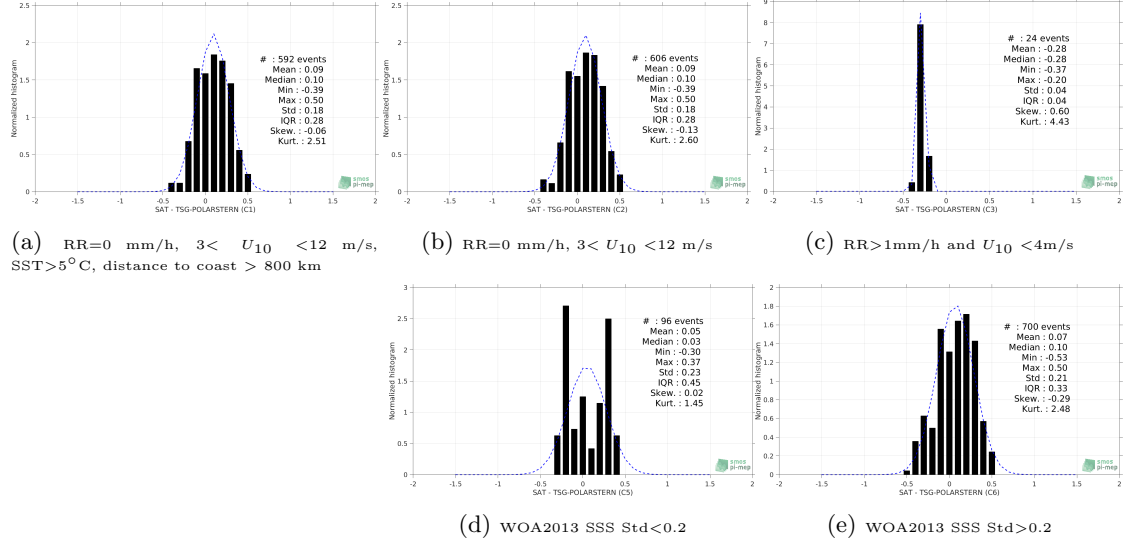
Figure 13: Normalized histogram of \Delta\text{SSS} (SMOS-L3-CATDS-CECOS-LOCEAN-V3-9DAYS-25KM - TSG-POLARSTERN) for 5 different subdatasets corresponding to: RR=0 mm/h, 3 < U_{10} < 12 m/s, SST > 5^\circ\text{C} , distance to coast > 800 km (a), RR=0 mm/h, 3 < U_{10} < 12 m/s (b), RR > 1\text{mm/h} and U_{10} < 4\text{m/s} (c), WOA2013 SSS Std <0.2 (d), WOA2013 SSS Std >0.2 (e).
