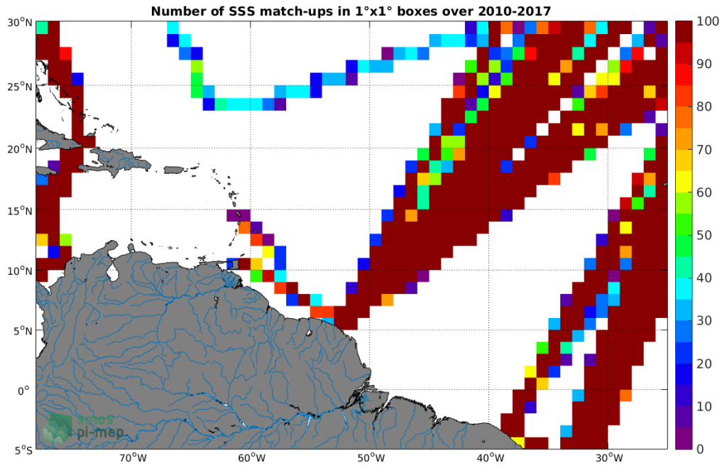
Figure 4: Number of SSS match-ups between TSG-LEGOS-DM SSS and the SMOS-L3-CATDS-CECOS-LOCEAN-V3-9DAYS-25KM SSS product for the Amazon and Orinoco river plumes Pi-MEP region over 1°x1° boxes and for the full satellite product period.
