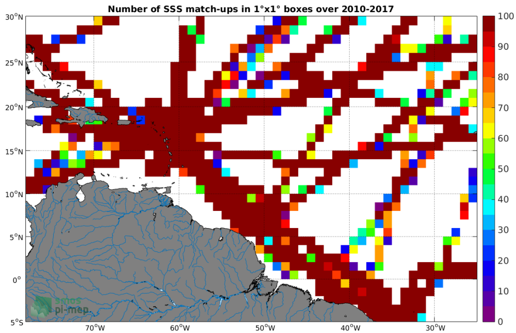
Figure 4: Number of SSS match-ups between TSG-GOSUD-Research-vessel SSS and the SMOS-L3-CATDS-CECOS-LOCEAN-V3-9DAYS-25KM SSS product for the Amazon and Orinoco river plumes Pi-MEP region over 1^\circ \times 1^\circ boxes and for the full satellite product period.
