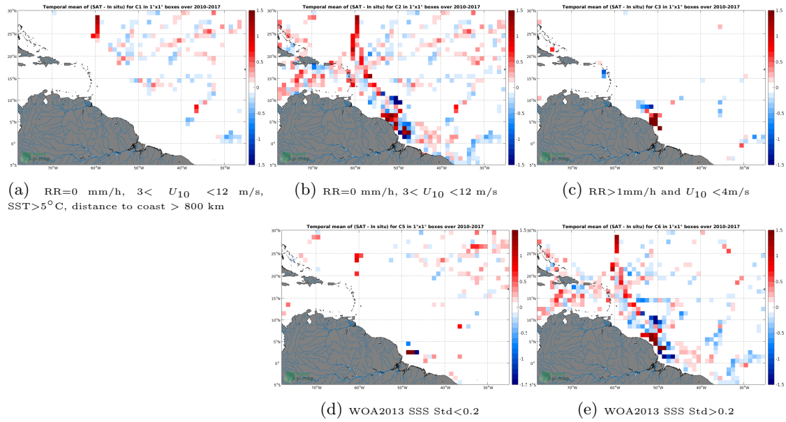
Figure 12: Temporal mean gridded over spatial boxes of size 1^\circ \times 1^\circ of \Delta SSS (SMOS-L3-CATDS-CECOS-LOCEAN-V3-9DAYS-25KM - TSG-GOSUD-Research-vessel) for 5 different subdatasets corresponding to: RR=0 mm/h, 3 < U_{10} < 12 m/s, SST > 5^\circ C , distance to coast > 800 km (a), RR=0 mm/h, 3 < U_{10} < 12 m/s (b), RR > 1 mm/h and U_{10} < 4 m/s (c), WOA2013 SSS Std < 0.2 (d), WOA2013 SSS Std > 0.2 (e).
