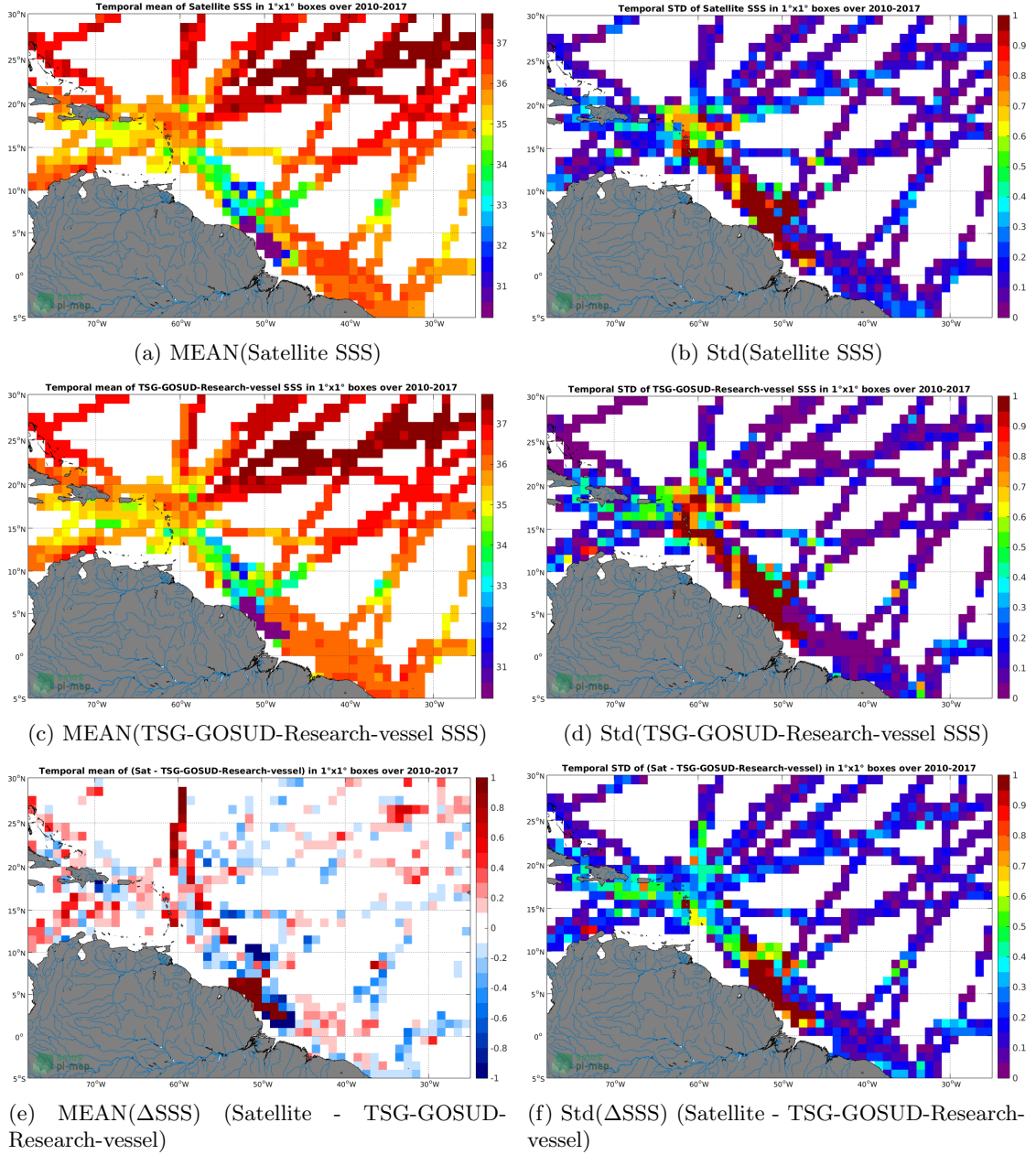
Figure 6: Temporal mean (left) and Std (right) of SSS from SMOS-L3-CATDS-CECOS-LOCEAN-V3-9DAYS-25KM (top), TSG-GOSUD-Research-vessel (middle), and of \Delta SSS (Satellite - TSG-GOSUD-Research-vessel). Only match-up pairs are used to generate these maps.
