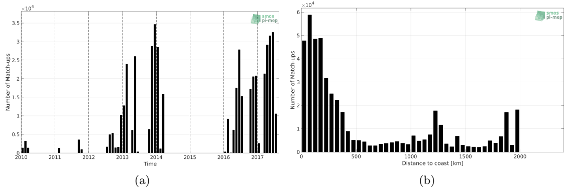
Figure 1: Number of match-ups between TSG-GOSUD-Research-vessel and SMOS-L3-CATDS-CECOS-LOCEAN-V3-9DAYS-25KM SSS as a function of time (a) and as function of the distance to coast (b) over the Amazon and Orinoco river plumes Pi-MEP region and for the full satellite product period.
