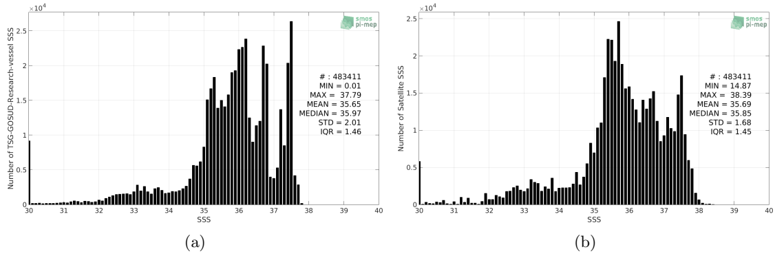
Figure 2: Histograms of SSS from TSG-GOSUD-Research-vessel (a) and SMOS-L3-CATDS-CECOS-LOCEAN-V3-9DAYS-25KM (b) considering all match-up pairs per bins of 0.1 over the Amazon and Orinoco river plumes Pi-MEP region and for the full satellite product period.
