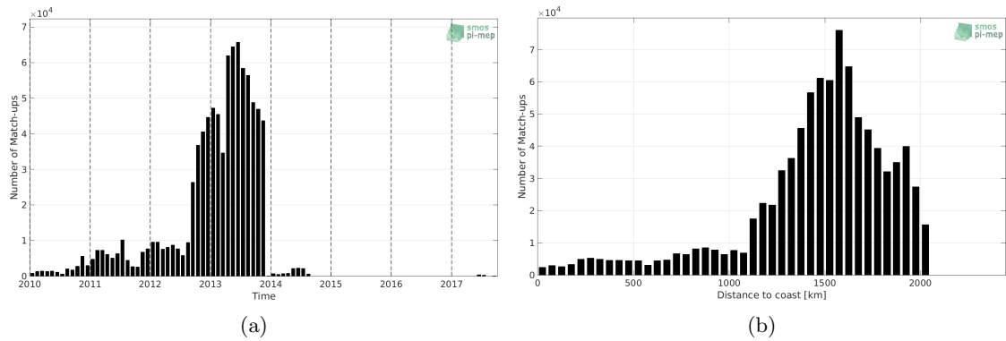
Figure 1: Number of match-ups between Surface drifters and SMOS-L3-CATDS-CECOS-LOCEAN-V3-9DAYS-25KM SSS as a function of time (a) and as function of the distance to coast (b) over the Amazon and Orinoco river plumes Pi-MEP region and for the full satellite product period.
