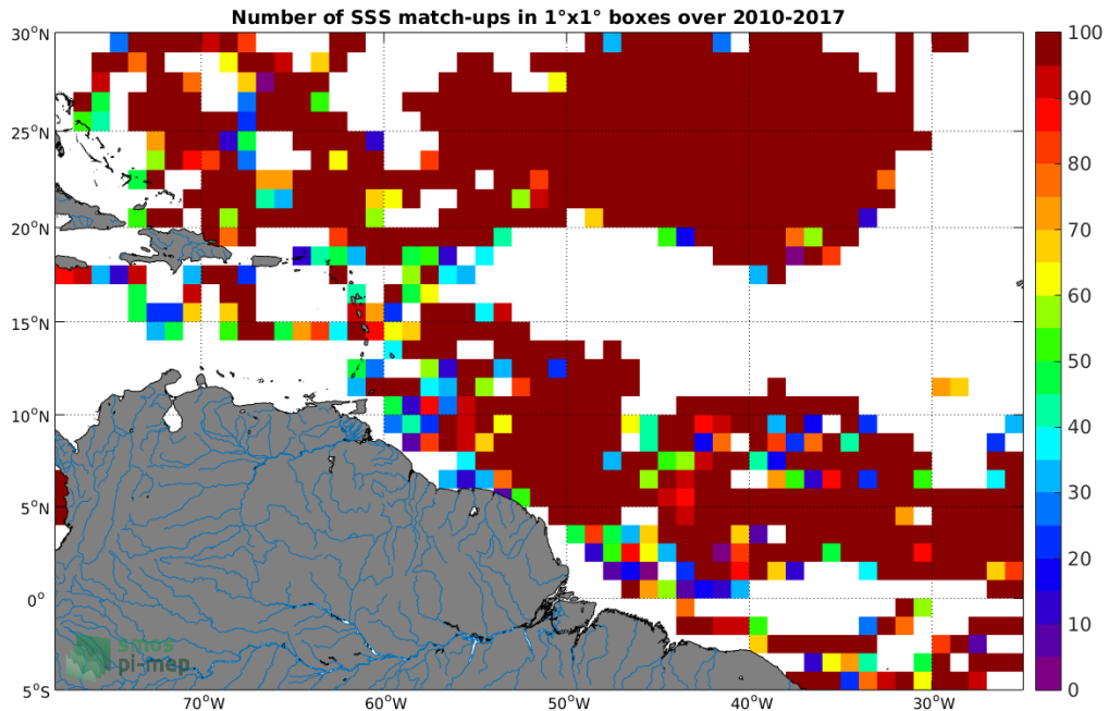
Figure 3: Number of SSS match-ups between Surface drifters SSS and the SMOS-L3-CATDS-CECOS-LOCEAN-V3-9DAYS-25KM SSS product for the Amazon and Orinoco river plumes Pi-MEP region over 1^\circ \times 1^\circ boxes and for the full satellite product period.
