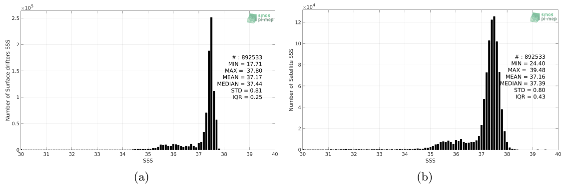
Figure 2: Histograms of SSS from Surface drifters (a) and SMOS-L3-CATDS-CECOS-LOCEAN-V3-9DAYS-25KM (b) considering all match-up pairs per bins of 0.1 over the Amazon and Orinoco river plumes Pi-MEP region and for the full satellite product period.
