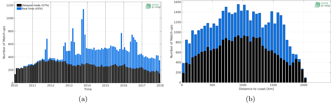
Figure 1: Number of match-ups between Argo and SMOS-L3-CATDS-CECOS-LOCEAN-V3-9DAYS-25KM SSS as a function of time (a) and as function of the distance to coast (b) over the Amazon and Orinoco river plumes Pi-MEP region and for the full satellite product period.
