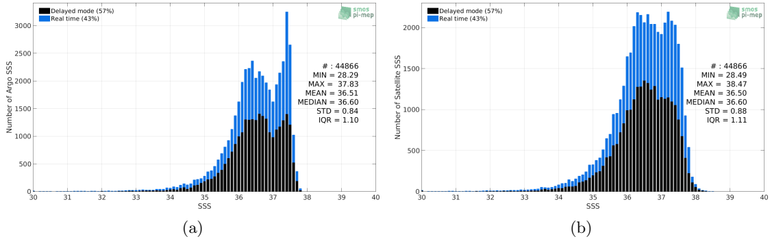
Figure 2: Histograms of SSS from Argo (a) and SMOS-L3-CATDS-CECOS-LOCEAN-V3-9DAYS-25KM (b) considering all match-up pairs per bins of 0.1 over the Amazon and Orinoco river plumes Pi-MEP region and for the full satellite product period.
