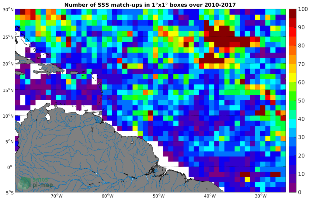
Figure 4: Number of SSS match-ups between Argo SSS and the SMOS-L3-CATDS-CECOS-LOCEAN-V3-9DAYS-25KM SSS product for the Amazon and Orinoco river plumes Pi-MEP region over 1°x1° boxes and for the full satellite product period.
