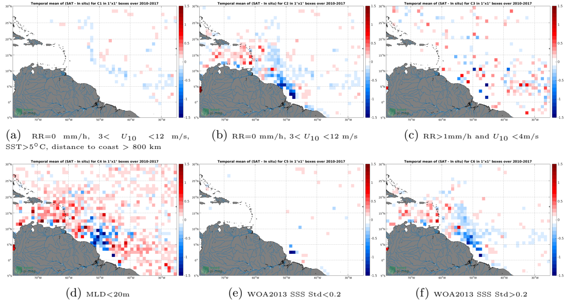
Figure 12: Temporal mean gridded over spatial boxes of size 1^\circ \times 1^\circ of \Delta SSS (SMOS-L3-CATDS-CECOS-LOCEAN-V3-18DAYS-25KM - Argo) for 6 different subdatasets corresponding to: RR=0 mm/h, 3 < U_{10} < 12 m/s, SST > 5^\circ\text{C} , distance to coast > 800 km (a), RR=0 mm/h, 3 < U_{10} < 12 m/s (b), RR > 1 mm/h and U_{10} < 4 m/s (c), MLD < 20 m (d), WOA2013 SSS Std < 0.2 (e), WOA2013 SSS Std > 0.2 (f).
