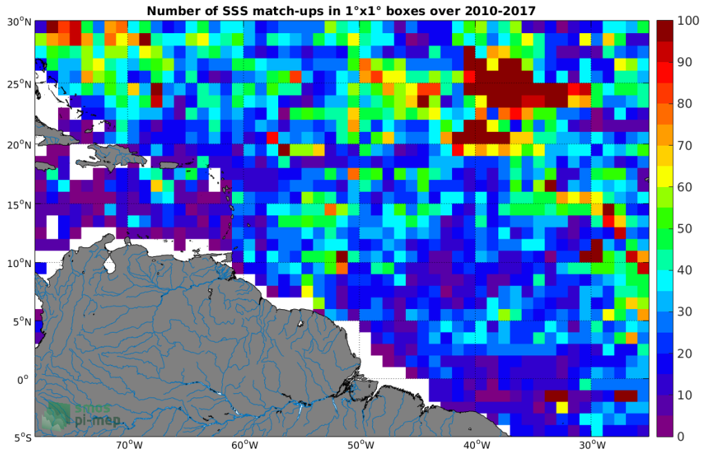
Figure 4: Number of SSS match-ups between Argos SSS and the SMOS-L3-CATDS-CECOS-LOCEAN-V3-18DAYS-25KM SSS product for the Amazon and Orinoco river plumes Pi-MEP region over 1^\circ \times 1^\circ boxes and for the full satellite product period.
