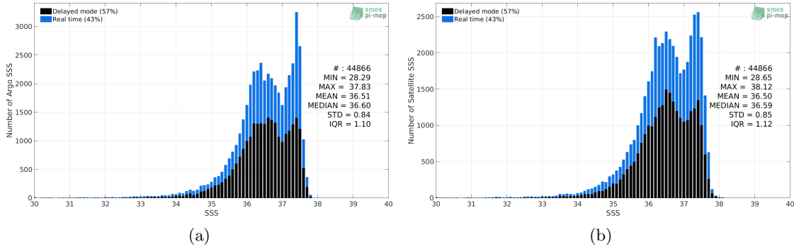
Figure 2: Histograms of SSS from Argo (a) and SMOS-L3-CATDS-CECOS-LOCEAN-V3-18DAYS-25KM (b) considering all match-up pairs per bins of 0.1 over the Amazon and Orinoco river plumes Pi-MEP region and for the full satellite product period.
