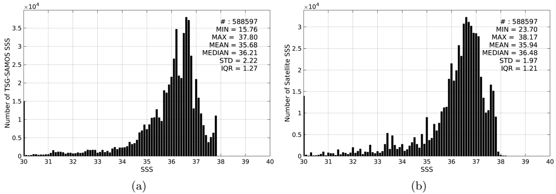
Figure 2: Histograms of SSS from TSG-SAMOS (a) and SMOS-L3-CATDS-CECOS-LOCEAN-V2-9DAYS-25KM (b) considering all match-up pairs per bins of 0.1 over the Amazon and Orinoco river plumes Pi-MEP region and for the full satellite product period.
