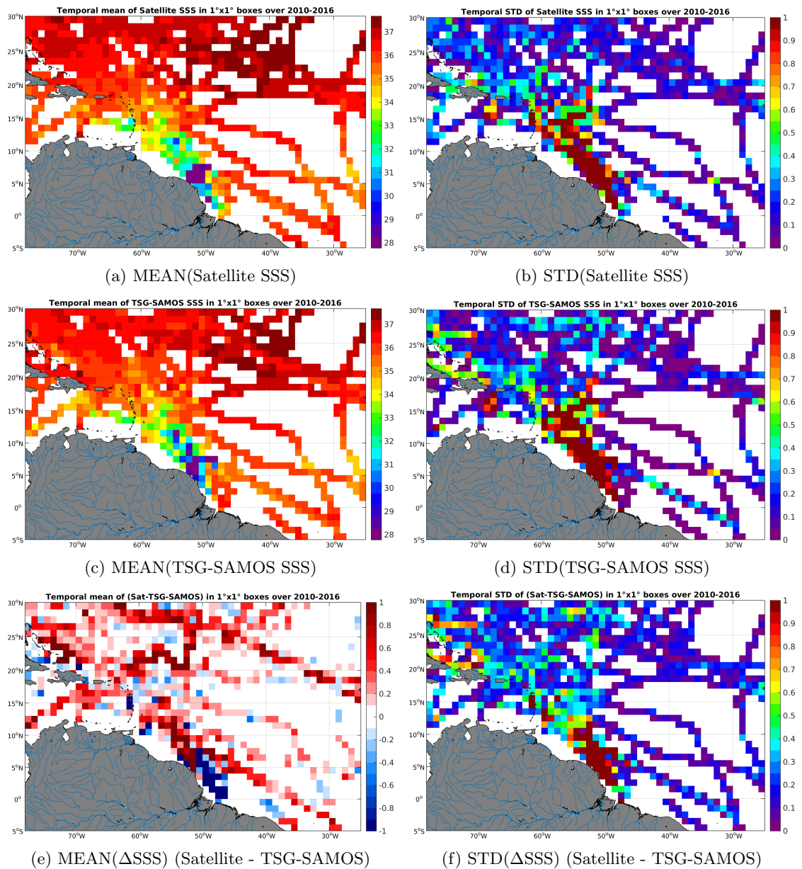
Figure 6: Temporal mean (left) and STD (right) of SSS from SMOS-L3-CATDS-CECOS-LOCEAN-V2-9DAYS-25KM (top), TSG-SAMOS (middle), and of \Delta SSS (Satellite - TSG-SAMOS). Only match-up pairs are used to generate these maps.
