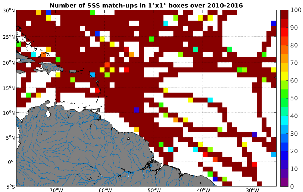
Figure 4: Number of SSS match-ups between TSG-SAMOS SSS and the SMOS-L3-CATDS-CECOS-LOCEAN-V2-9DAYS-25KM SSS product for the Amazon and Orinoco river plumes Pi-MEP region over 1^\circ \times 1^\circ boxes and for the full satellite product period.
