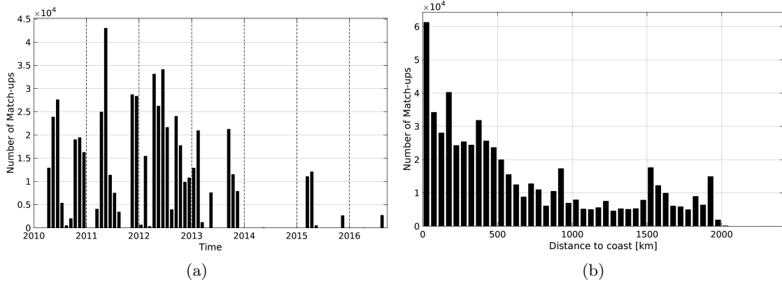
Figure 1: Number of match-ups between TSG-SAMOS and SMOS-L3-CATDS-CECOS-LOCEAN-V2-9DAYS-25KM SSS as a function of time (a) and as function of the distance to coast (b) over the Amazon and Orinoco river plumes Pi-MEP region and for the full satellite product period.
