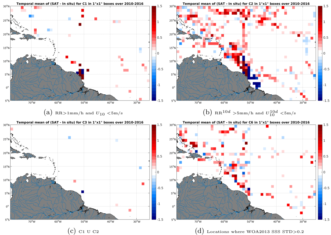
Figure 12: Temporal mean gridded over spatial boxes of size 1^\circ \times 1^\circ of \Delta SSS (SMOS-L3-CATDS-CECOS-LOCEAN-V2-9DAYS-25KM - TSG-SAMOS) for 4 different subdatasets corresponding to:RR >1 mm/h and U_{10} < 5 m/s (a), RR ^{10d} > 5 mm/h and U_{10}^{10d} < 5 m/s (b), C1 U C2 (c),Locations where WOA2013 SSS STD >0.2 (d).
