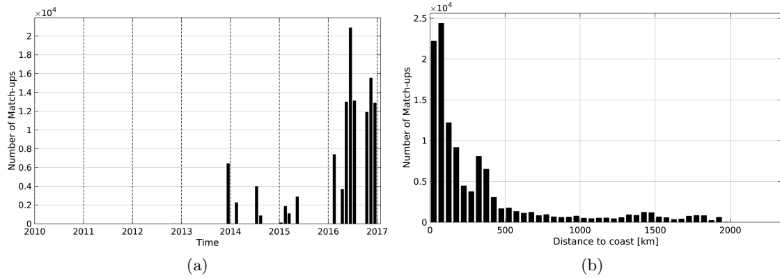
Figure 1: Number of match-ups between TSG-GOSUD-Sailing-ship and SMOS-L3-CATDS-CECOS-LOCEAN-V2-9DAYS-25KM SSS as a function of time (a) and as function of the distance to coast (b) over the Amazon and Orinoco river plumes Pi-MEP region and for the full satellite product period.
