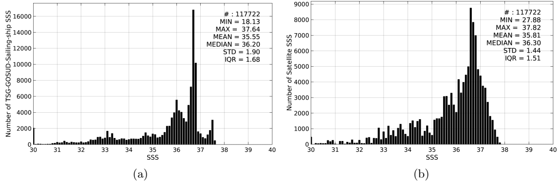
Figure 2: Histograms of SSS from TSG-GOSUD-Sailing-ship (a) and SMOS-L3-CATDS-CECOS-LOCEAN-V2-9DAYS-25KM (b) considering all match-up pairs per bins of 0.1 over the Amazon and Orinoco river plumes Pi-MEP region and for the full satellite product period.
