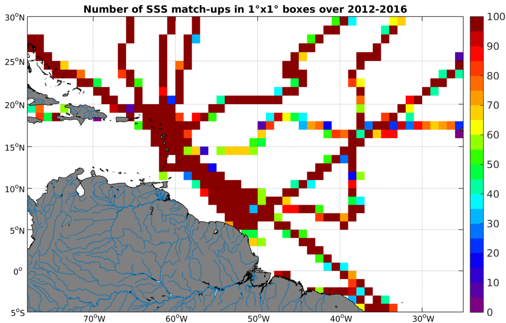
Figure 4: Number of SSS match-ups between TSG-GOSUD-Sailing-ship SSS and the SMOS-L3-CATDS-CECOS-LOCEAN-V2-9DAYS-25KM SSS product for the Amazon and Orinoco river plumes Pi-MEP region over 1^\circ \times 1^\circ boxes and for the full satellite product period.
