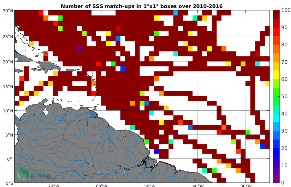
Figure 4: Number of SSS match-ups between TSG-SAMOS SSS and the SMOS-L3-CATDS-IFREMER-CECOS-V2-MONTHLY-0.25DEG SSS product for the Amazon and Orinoco river plumes Pi-MEP region over 1^\circ \times 1^\circ boxes and for the full satellite product period.
