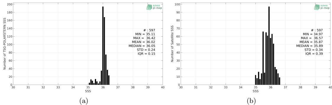
Figure 2: Histograms of SSS from TSG-POLARSTERN (a) and SMOS L3 v2 - Monthly - 0.25 Deg (CATDS-CECOS-IFREMER) (b) considering all match-up pairs per bins of 0.1 over the Amazon and Orinoco river plumes Pi-MEP region and for the full satellite product period.
