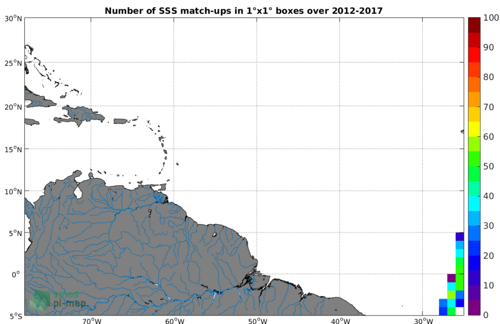
Figure 4: Number of SSS match-ups between TSG-POLARSTERN SSS and the SMOS L3 v2 - Monthly - 0.25 Deg (CATDS-CECOS-IFREMER) SSS product for the Amazon and Orinoco river plumes Pi-MEP region over 1°x1° boxes and for the full satellite product period.
