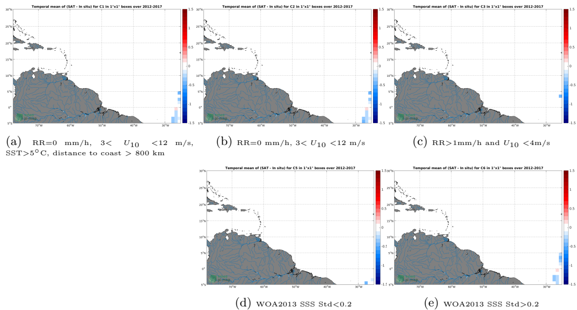
Figure 12: Temporal mean gridded over spatial boxes of size 1^{\circ}\times 1^{\circ} of \Delta\text{SSS} (SMOS L3 v2 - Monthly - 0.25 Deg (CATDS-CECOS-IFREMER) - TSG-POLARSTERN) for 5 different sub-datasets corresponding to:RR=0 mm/h, 3 < U_{10} < 12 m/s, SST >5^{\circ}\text{C} , distance to coast > 800 km (a), RR=0 mm/h, 3 < U_{10} < 12 m/s (b), RR >1 mm/h and U_{10} < 4 m/s (c), WOA2013 SSS Std <0.2 (d), WOA2013 SSS Std >0.2 (e).
