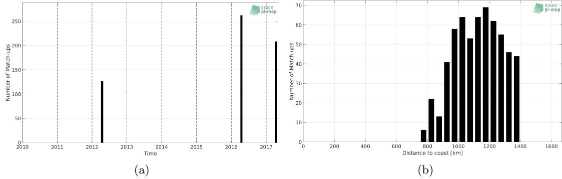
Figure 1: Number of match-ups between TSG-POLARSTERN and SMOS L3 v2 - Monthly - 0.25 Deg (CATDS-CECOS-IFREMER) SSS as a function of time (a) and as function of the distance to coast (b) over the Amazon and Orinoco river plumes Pi-MEP region and for the full satellite product period.
