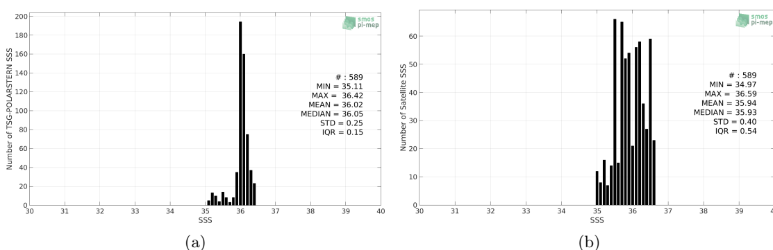
Figure 2: Histograms of SSS from TSG-POLARSTERN (a) and SMOS-L3-CATDS-IFREMER-CECOS-V2-MONTHLY-0.25DEG (b) considering all match-up pairs per bins of 0.1 over the Amazon and Orinoco river plumes Pi-MEP region and for the full satellite product period.
