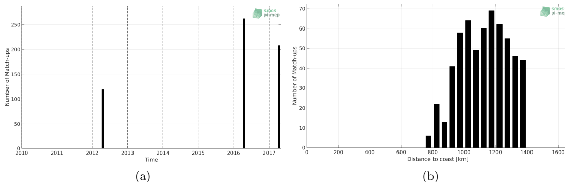
Figure 1: Number of match-ups between TSG-POLARSTERN and SMOS-L3-CATDS-IFREMER-CECOS-V2-MONTHLY-0.25DEG SSS as a function of time (a) and as function of the distance to coast (b) over the Amazon and Orinoco river plumes Pi-MEP region and for the full satellite product period.
