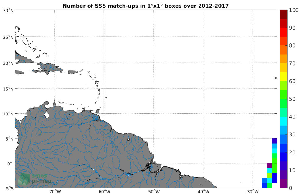
Figure 4: Number of SSS match-ups between TSG-POLARSTERN SSS and the SMOS-L3-CATDS-IFREMER-CECOS-V2-MONTHLY-0.25DEG SSS product for the Amazon and Orinoco river plumes Pi-MEP region over 1^\circ \times 1^\circ boxes and for the full satellite product period.
