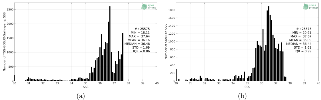
Figure 2: Histograms of SSS from TSG-GOSUD-Sailing-ship (a) and SMOS L3 v2 - Monthly - 0.25 Deg (CATDS-CECOS-IFREMER) (b) considering all match-up pairs per bins of 0.1 over the Amazon and Orinoco river plumes Pi-MEP region and for the full satellite product period.
