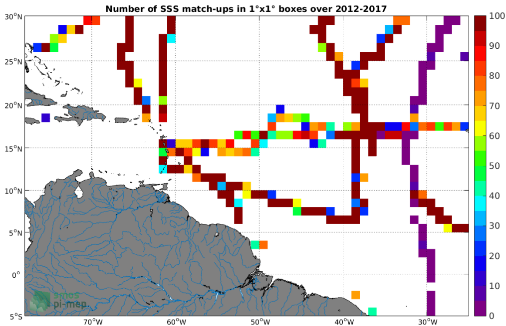
Figure 4: Number of SSS match-ups between TSG-GOSUD-Sailing-ship SSS and the SMOS L3 v2 - Monthly - 0.25 Deg (CATDS-CECOS-IFREMER) SSS product for the Amazon and Orinoco river plumes Pi-MEP region over 1°x1° boxes and for the full satellite product period.
