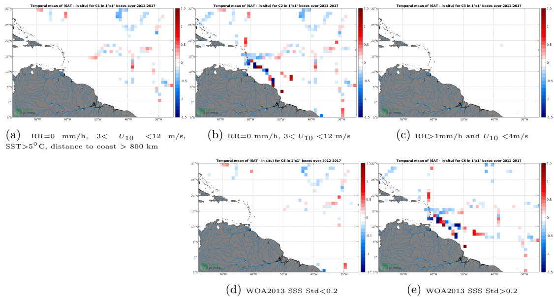
Figure 12: Temporal mean gridded over spatial boxes of size 1^{\circ}\times 1^{\circ} of \Delta SSS (SMOS L3 v2 - Monthly - 0.25 Deg (CATDS-CECOS-IFREMER) - TSG-GOSUD-Sailing-ship) for 5 different subdatasets corresponding to:RR=0 mm/h, 3 < U_{10} < 12 m/s, SST >5^{\circ}\text{C} , distance to coast > 800 km (a), RR=0 mm/h, 3 < U_{10} < 12 m/s (b), RR >1 mm/h and U_{10} < 4 m/s (c), WOA2013 SSS Std <0.2 (d), WOA2013 SSS Std >0.2 (e).
