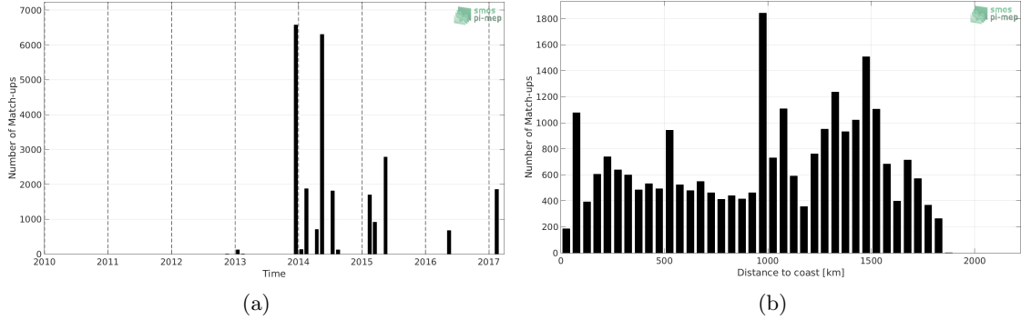
Figure 1: Number of match-ups between TSG-GOSUD-Sailing-ship and SMOS-L3-CATDS-IFREMER-CECOS-V2-MONTHLY-0.25DEG SSS as a function of time (a) and as function of the distance to coast (b) over the Amazon and Orinoco river plumes Pi-MEP region and for the full satellite product period.
