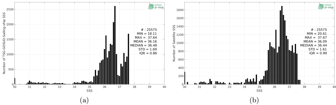
Figure 2: Histograms of SSS from TSG-GOSUD-Sailing-ship (a) and SMOS-L3-CATDS-IFREMER-CECOS-V2-MONTHLY-0.25DEG (b) considering all match-up pairs per bins of 0.1 over the Amazon and Orinoco river plumes Pi-MEP region and for the full satellite product period.
