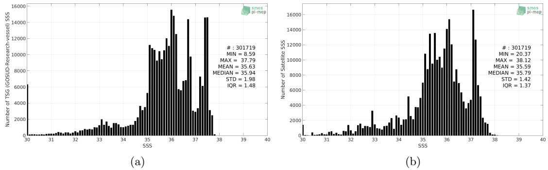
Figure 2: Histograms of SSS from TSG (GOSUD-Research-vessel) (a) and SMOS SSS L3 v2 - Monthly - 0.25 Deg (CATDS-CECOS-IFREMER) (b) considering all match-up pairs per bins of 0.1 over the Amazon and Orinoco river plumes Pi-MEP region and for the full satellite product period.
