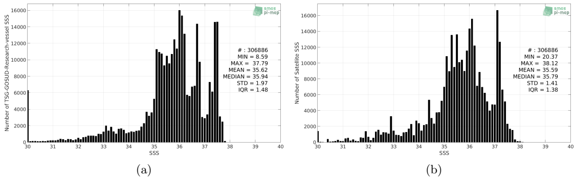
Figure 2: Histograms of SSS from TSG-GOSUD-Research-vessel (a) and SMOS L3 v2 - Monthly - 0.25 Deg (CATDS-CECOS-IFREMER) (b) considering all match-up pairs per bins of 0.1 over the Amazon and Orinoco river plumes Pi-MEP region and for the full satellite product period.
