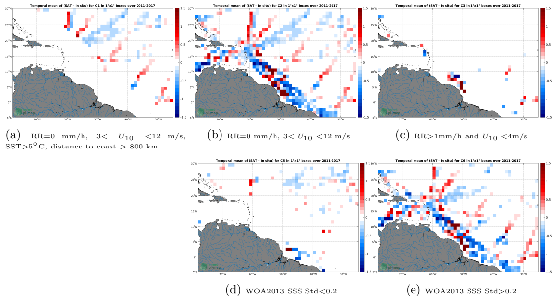
Figure 12: Temporal mean gridded over spatial boxes of size 1^{\circ}\times 1^{\circ} of \Delta SSS (SMOS L3 v2 - Monthly - 0.25 Deg (CATDS-CECOS-IFREMER) - TSG-GOSUD-Research-vessel) for 5 different subdatasets corresponding to:RR=0 mm/h, 3 < U_{10} < 12 m/s, SST >5^{\circ}\text{C} , distance to coast > 800 km (a), RR=0 mm/h, 3 < U_{10} < 12 m/s (b), RR >1 mm/h and U_{10} < 4 m/s (c), WOA2013 SSS Std <0.2 (d), WOA2013 SSS Std >0.2 (e).
