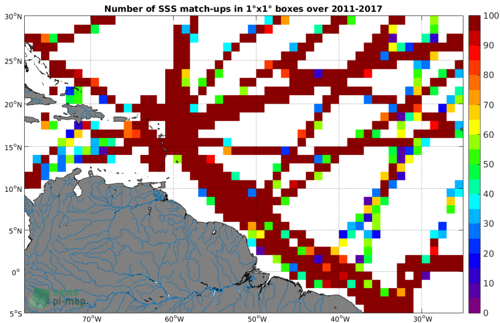
Figure 4: Number of SSS match-ups between TSG-GOSUD-Research-vessel SSS and the SMOS L3 v2 - Monthly - 0.25 Deg (CATDS-CECOS-IFREMER) SSS product for the Amazon and Orinoco river plumes Pi-MEP region over 1°x1° boxes and for the full satellite product period.
