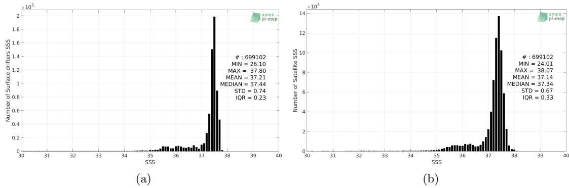
Figure 2: Histograms of SSS from Surface drifters (a) and SMOS L3 v2 - Monthly - 0.25 Deg (CATDS-CECOS-IFREMER) (b) considering all match-up pairs per bins of 0.1 over the Amazon and Orinoco river plumes Pi-MEP region and for the full satellite product period.
