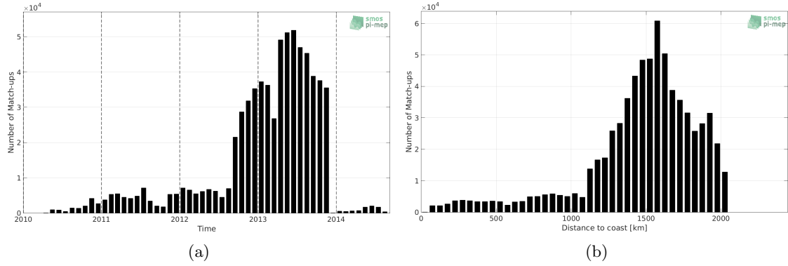
Figure 1: Number of match-ups between Surface drifters and SMOS L3 v2 - Monthly - 0.25 Deg (CATDS-CECOS-IFREMER) SSS as a function of time (a) and as function of the distance to coast (b) over the Amazon and Orinoco river plumes Pi-MEP region and for the full satellite product period.
