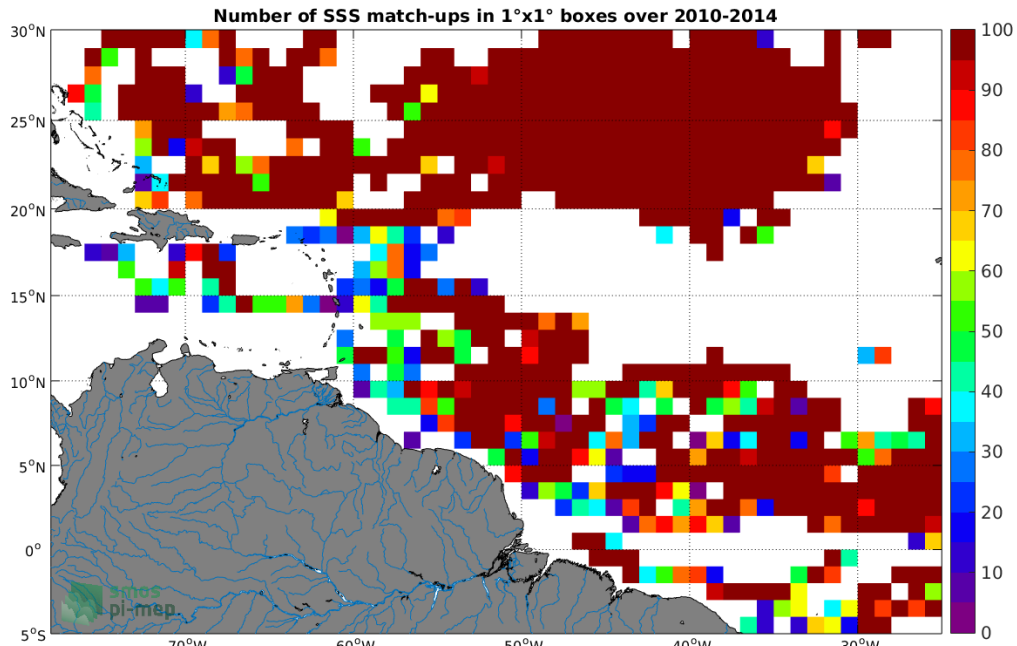
Figure 3: Number of SSS match-ups between Surface drifters SSS and the SMOS L3 v2 - Monthly - 0.25 Deg (CATDS-CECOS-IFREMER) SSS product for the Amazon and Orinoco river plumes Pi-MEP region over 1°x1° boxes and for the full satellite product period.
