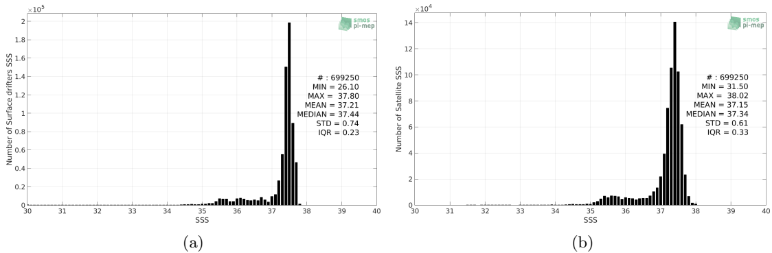
Figure 2: Histograms of SSS from Surface drifters (a) and SMOS-L3-CATDS-IFREMER-CECOS-V2-MONTHLY-0.25DEG (b) considering all match-up pairs per bins of 0.1 over the Amazon and Orinoco river plumes Pi-MEP region and for the full satellite product period.
