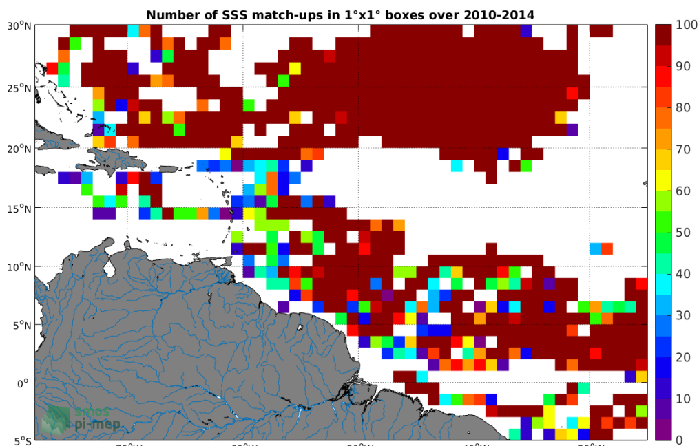
Figure 3: Number of SSS match-ups between Surface drifters SSS and the SMOS-L3-CATDS-IFREMER-CECOS-V2-MONTHLY-0.25DEG SSS product for the Amazon and Orinoco river plumes Pi-MEP region over 1°x1° boxes and for the full satellite product period.
