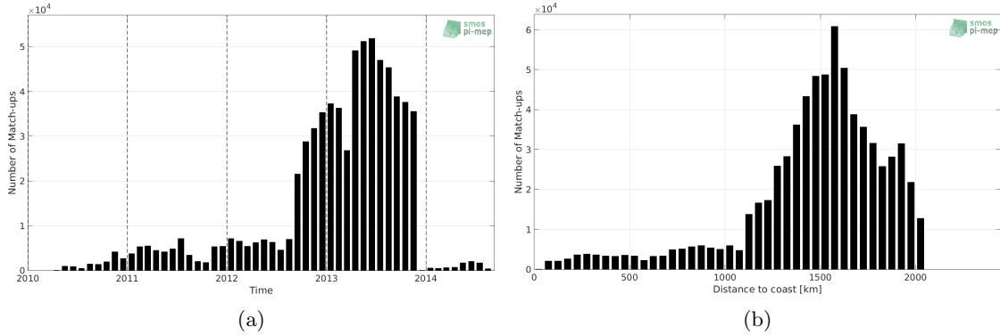
Figure 1: Number of match-ups between Surface drifters and SMOS-L3-CATDS-IFREMER-CECOS-V2-MONTHLY-0.25DEG SSS as a function of time (a) and as function of the distance to coast (b) over the Amazon and Orinoco river plumes Pi-MEP region and for the full satellite product period.
