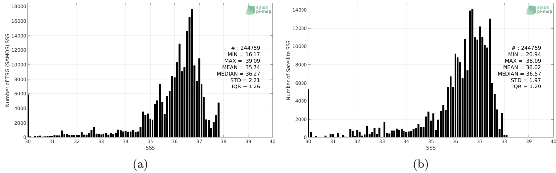
Figure 2: Histograms of SSS from TSG (SAMOS) (a) and SMOS SSS L3 v2 - Daily - 0.5 Deg (CATDS-CECOS-IFREMER) (b) considering all match-up pairs per bins of 0.1 over the Amazon and Orinoco river plumes Pi-MEP region and for the full satellite product period.
