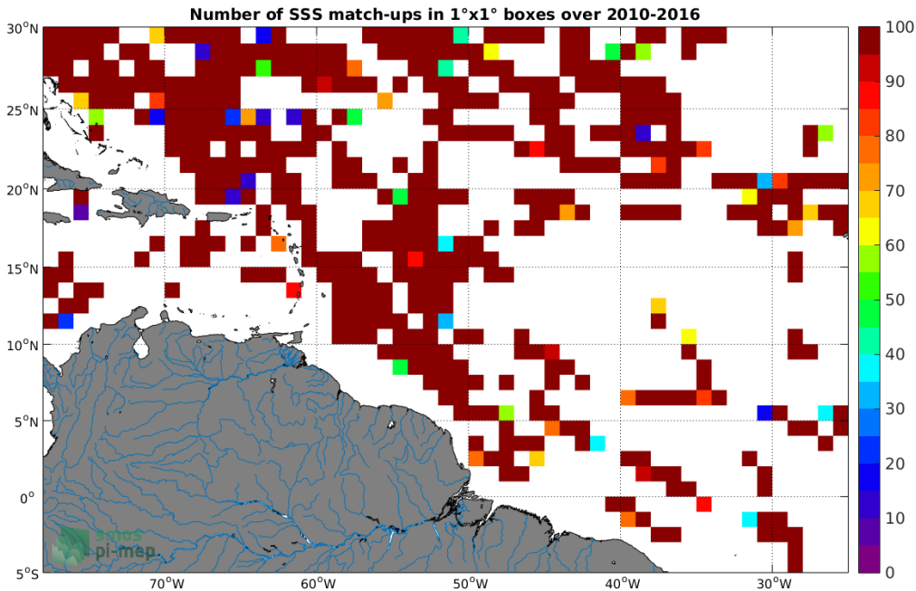
Figure 4: Number of SSS match-ups between TSG-SAMOS SSS and the SMOS L3 v2 - Daily - 0.5 Deg (CATDS-CECOS-IFREMER) SSS product for the Amazon and Orinoco river plumes Pi-MEP region over 1°x1° boxes and for the full satellite product period.
