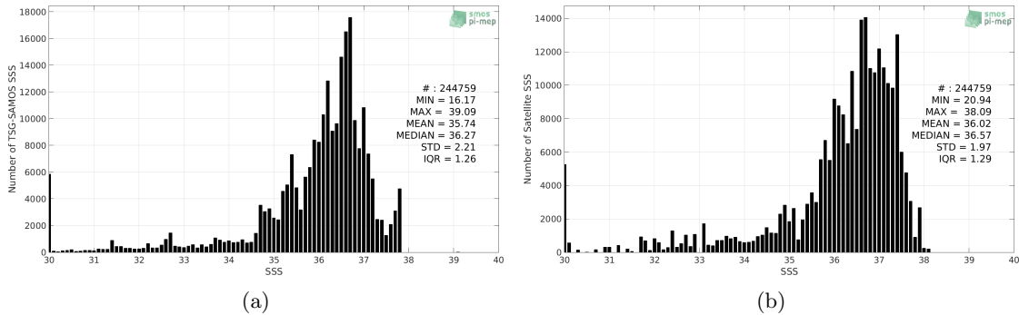
Figure 2: Histograms of SSS from TSG-SAMOS (a) and SMOS L3 v2 - Daily - 0.5 Deg (CATDS-CECOS-IFREMER) (b) considering all match-up pairs per bins of 0.1 over the Amazon and Orinoco river plumes Pi-MEP region and for the full satellite product period.
