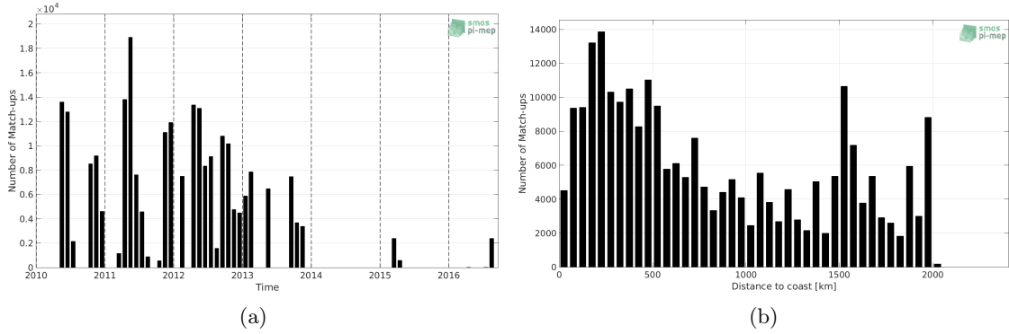
Figure 1: Number of match-ups between TSG-SAMOS and SMOS L3 v2 - Daily - 0.5 Deg (CATDS-CECOS-IFREMER) SSS as a function of time (a) and as function of the distance to coast (b) over the Amazon and Orinoco river plumes Pi-MEP region and for the full satellite product period.
