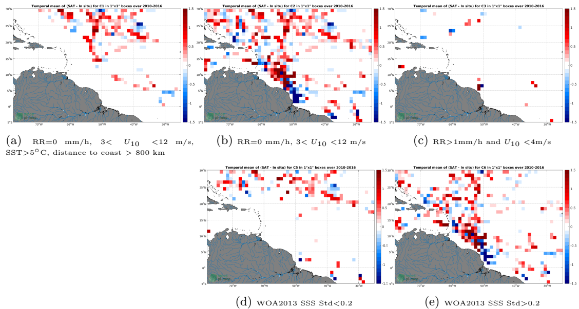
Figure 12: Temporal mean gridded over spatial boxes of size 1^\circ \times 1^\circ of \Delta SSS (SMOS L3 v2 - Daily - 0.5 Deg (CATDS-CECOS-IFREMER) - TSG-SAMOS) for 5 different subdatasets corresponding to:RR=0 mm/h, 3 < U_{10} < 12 m/s, SST >5^\circ\text{C} , distance to coast > 800 km (a), RR=0 mm/h, 3 < U_{10} < 12 m/s (b), RR >1 mm/h and U_{10} < 4 m/s (c), WOA2013 SSS Std <0.2 (d), WOA2013 SSS Std >0.2 (e).
