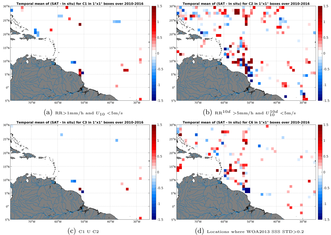
Figure 12: Temporal mean gridded over spatial boxes of size 1^\circ \times 1^\circ of \Delta SSS (SMOS-L3-CATDS-CECOS-IFREMER-V2-1DAY-0.5deg - TSG-SAMOS) for 4 different subdatasets corresponding to:RR>1mm/h and U_{10} < 5\text{m/s} (a), RR^{10d} > 5\text{mm/h} and U_{10}^{10d} < 5\text{m/s} (b), C1 U C2 (c),Locations where WOA2013 SSS STD>0.2 (d).
