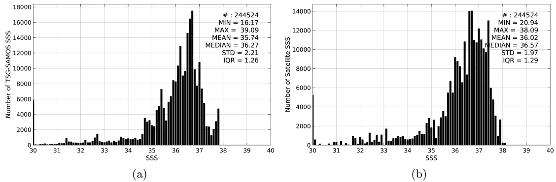
Figure 2: Histograms of SSS from TSG-SAMOS (a) and SMOS-L3-CATDS-CECOS-IFREMER-V2-1DAY-0.5deg (b) considering all match-up pairs per bins of 0.1 over the Amazon and Orinoco river plumes Pi-MEP region and for the full satellite product period.
